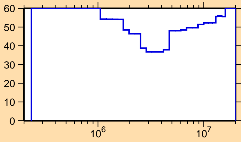
\Delta\sigma/\sigma vs. E for ^{76}\text{Sr}(n,n_1)
