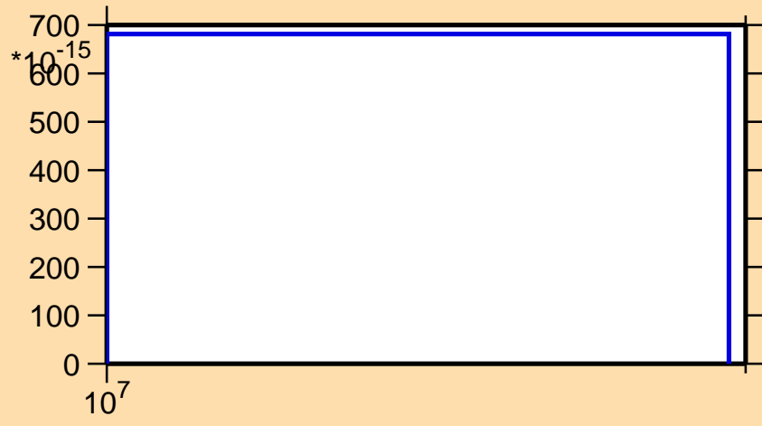
\sigma vs. E for ^{76}\text{Sr} (mt 34)
