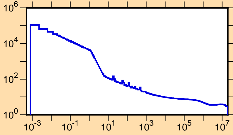
\sigma vs. E for ^{77}\text{Sr}(n,\text{tot.})
