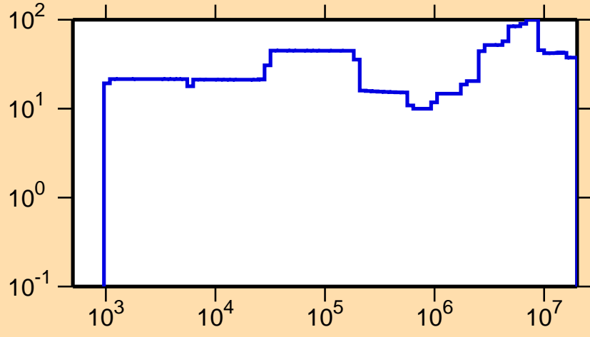
\Delta\sigma/\sigma vs. E for ^{77}\text{Sr}(n,p)
