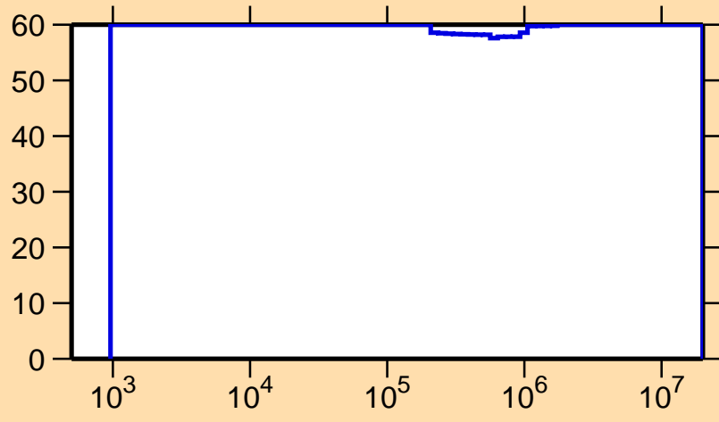
\Delta\sigma/\sigma vs. E for ^{77}\text{Sr}(n,\gamma)
