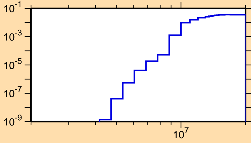
\sigma vs. E for ^{77}\text{Sr}(n,d)
