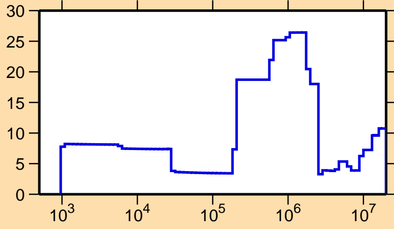
\Delta\sigma/\sigma vs. E for ^{77}\text{Sr}(n,\text{el.})
