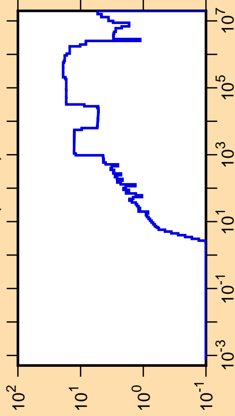
\Delta\sigma/\sigma vs. E for ^{77}\text{Sr}(n,\text{tot.})
