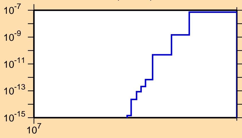
\sigma vs. E for ^{77}\text{Sr}(\text{mt } 34)
