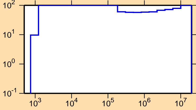
\Delta\sigma/\sigma vs. E for ^{77}\text{Sr}(n,\gamma)
