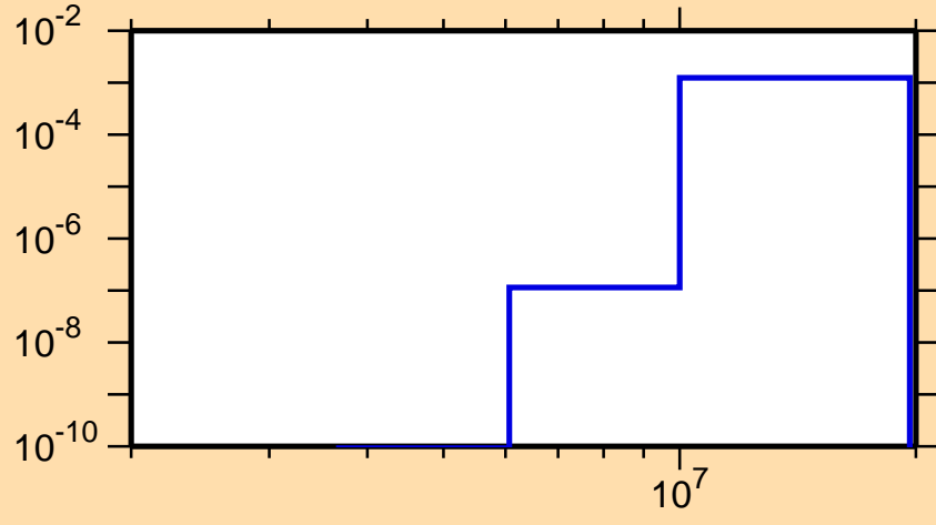
\sigma vs. E for ^{77}\text{Sr}(n,\text{He}3)
