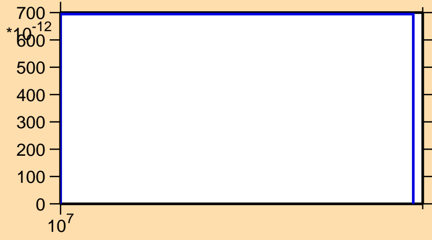
\sigma vs. E for ^{77}\text{Sr} (mt 34)
