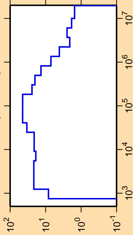
\Delta\sigma/\sigma vs. E for ^{77}\text{Sr}(n,\text{nonel.})
