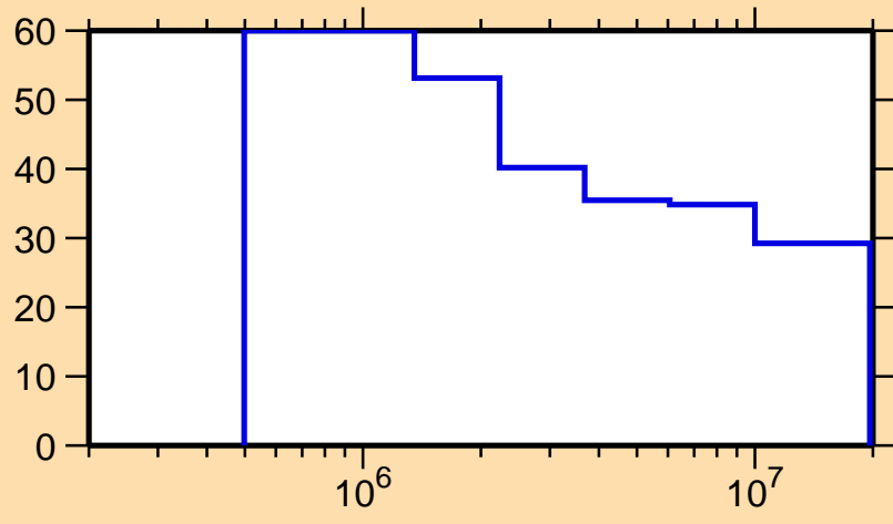
\Delta\sigma/\sigma vs. E for ^{77}\text{Sr}(n,n_1)
