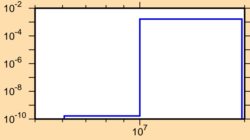
\sigma vs. E for ^{77}\text{Sr}(n,\text{pd})
