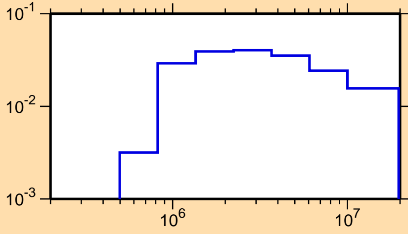
\sigma vs. E for ^{77}\text{Sr}(n,n_3)
