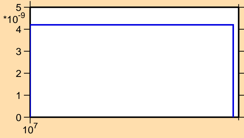
\sigma vs. E for ^{77}\text{Sr} (mt 45)
