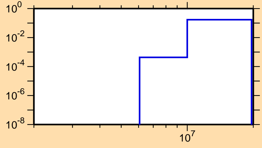
\sigma vs. E for ^{77}\text{Sr}(n,np)
