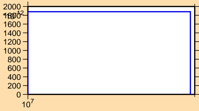
\sigma vs. E for ^{77}\text{Sr}(n,\text{nd})
