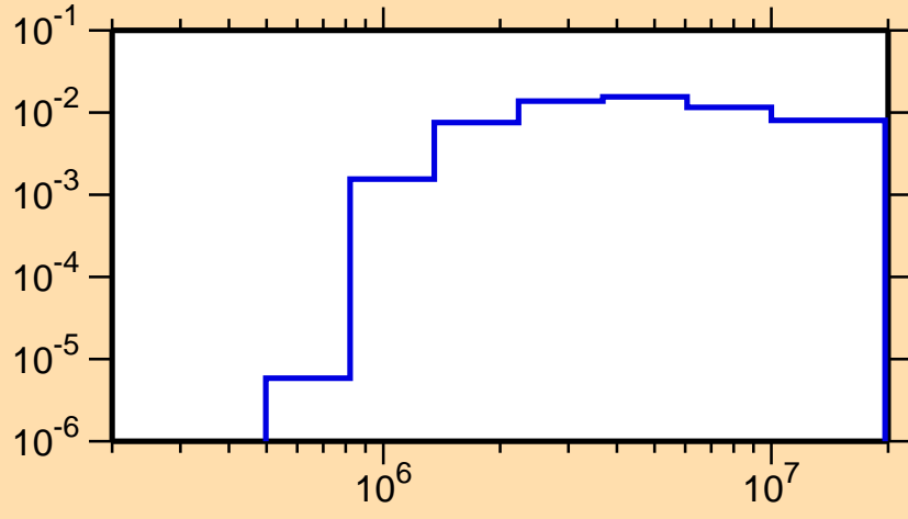
\sigma vs. E for ^{77}\text{Sr}(n,n\text{cont.})
