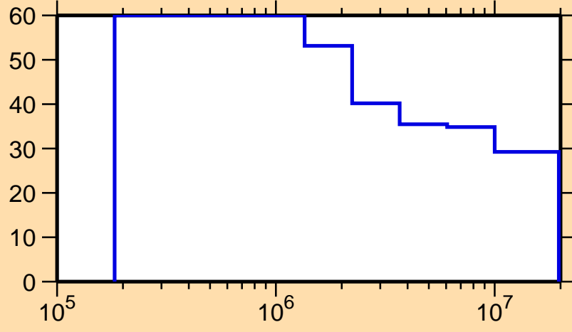
\Delta\sigma/\sigma vs. E for ^{77}\text{Sr}(n,n_1)
