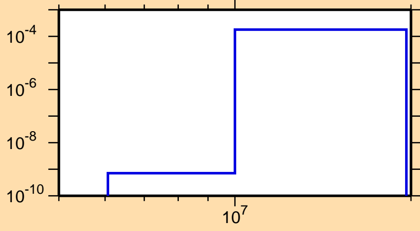
\sigma vs. E for ^{77}\text{Sr}(n,\alpha)
