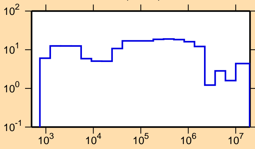
\Delta\sigma/\sigma vs. E for ^{77}\text{Sr}(n,\text{tot.})
