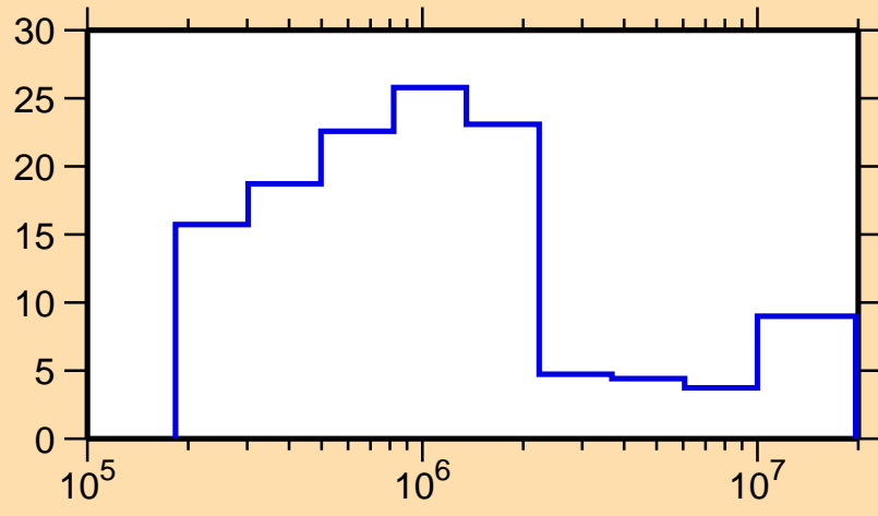
\Delta\sigma/\sigma vs. E for ^{77}\text{Sr}(n,\text{el.})
