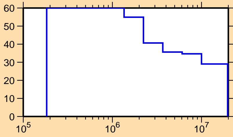
\Delta\sigma/\sigma vs. E for ^{77}\text{Sr}(n,\text{inel.})
