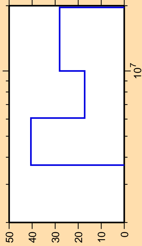
\Delta\sigma/\sigma vs. E for ^{77}\text{Sr}(n,np)
