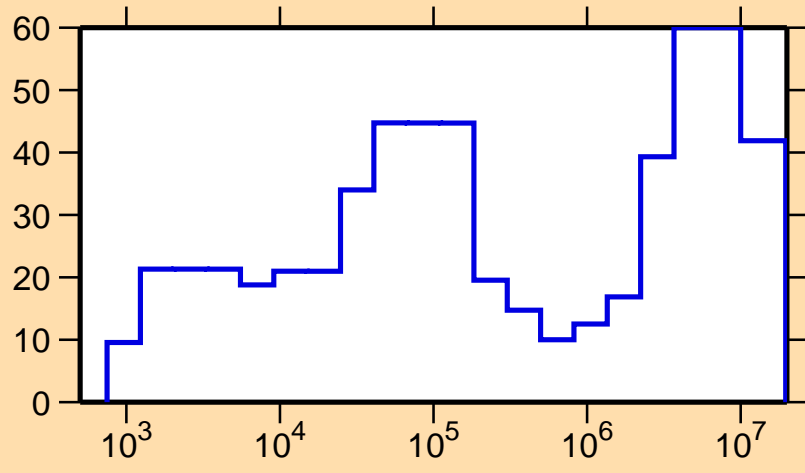
\Delta\sigma/\sigma vs. E for ^{77}\text{Sr}(n,p)
