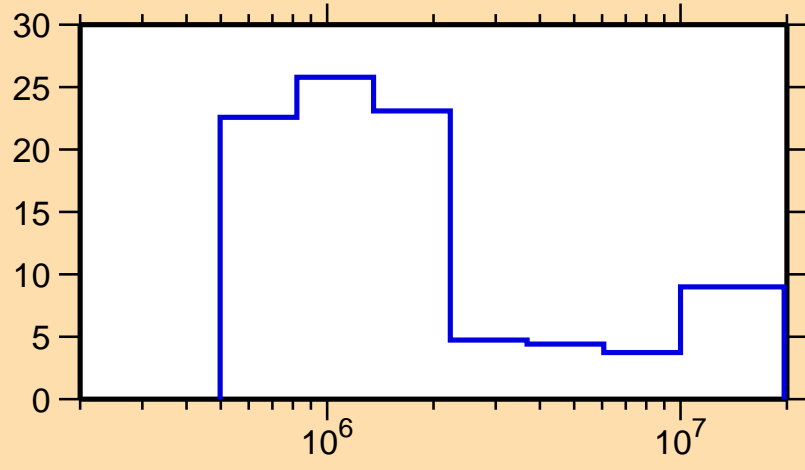
\Delta\sigma/\sigma vs. E for ^{77}\text{Sr}(n,el.)
