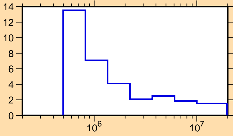
\Delta\sigma/\sigma vs. E for ^{77}\text{Sr}(n,\text{nonel.})
