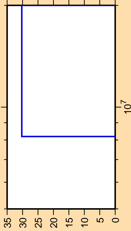
\Delta\sigma/\sigma vs. E for ^{77}\text{Sr}(n,n_1)
