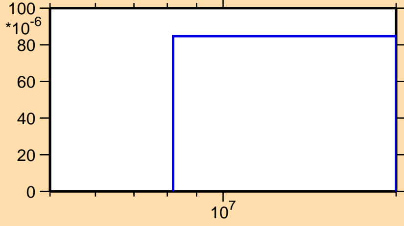
\sigma vs. E for ^{77}\text{Sr}(n,t)
