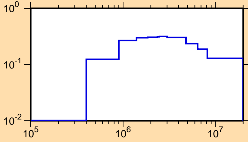
\sigma vs. E for ^{77}\text{Sr}(n,\text{inel.})
