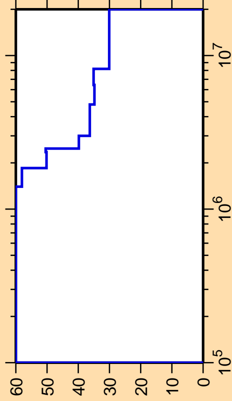
\Delta\sigma/\sigma vs. E for ^{77}\text{Sr}(n,\text{inel.})
