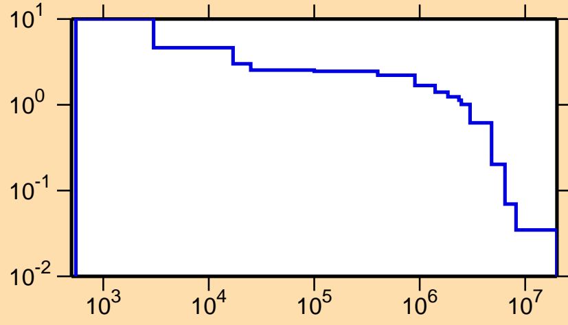
\sigma vs. E for ^{77}\text{Sr}(n,p)
