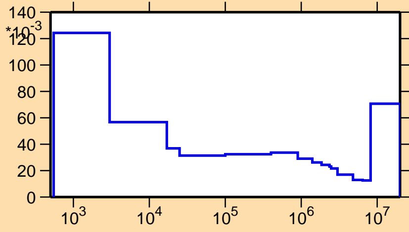
\sigma vs. E for ^{77}\text{Sr}(n,\alpha)
