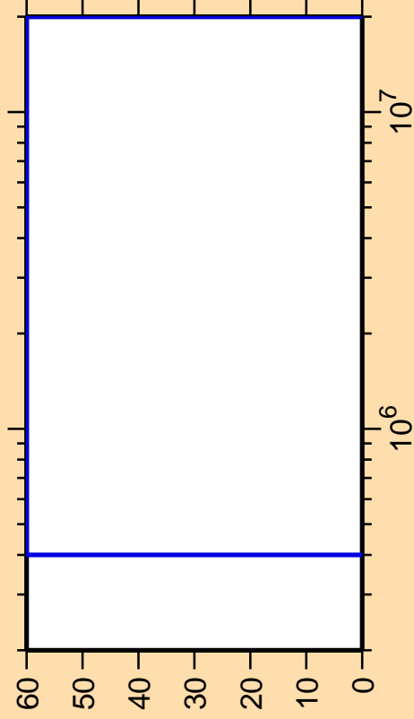
\Delta\sigma/\sigma vs. E for ^{77}\text{Sr}(n,\text{ncont.})
