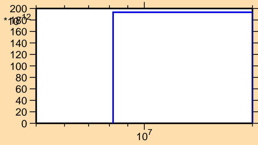
\sigma vs. E for ^{77}\text{Sr}(n,2np)
