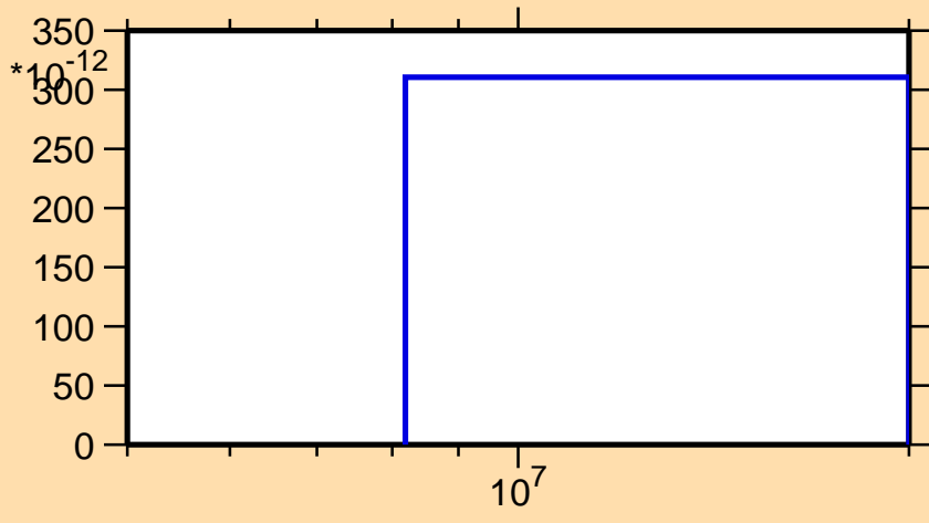
\sigma vs. E for ^{77}\text{Sr}(\text{mt117})
