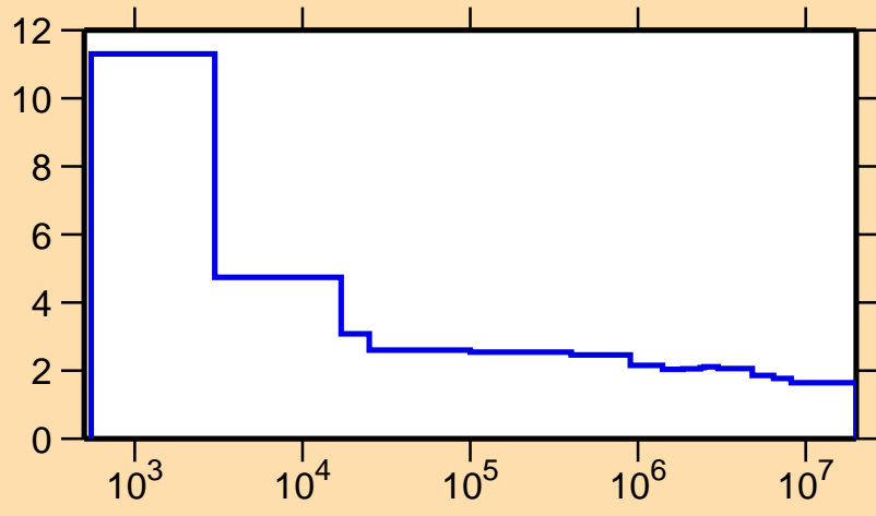
\sigma vs. E for ^{77}\text{Sr}(n,\text{nonel.})
