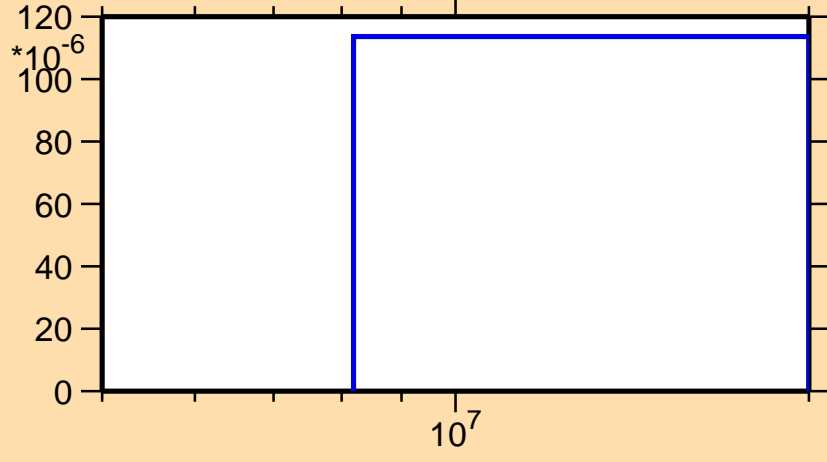
\sigma vs. E for ^{77}\text{Sr}(n,2n)
