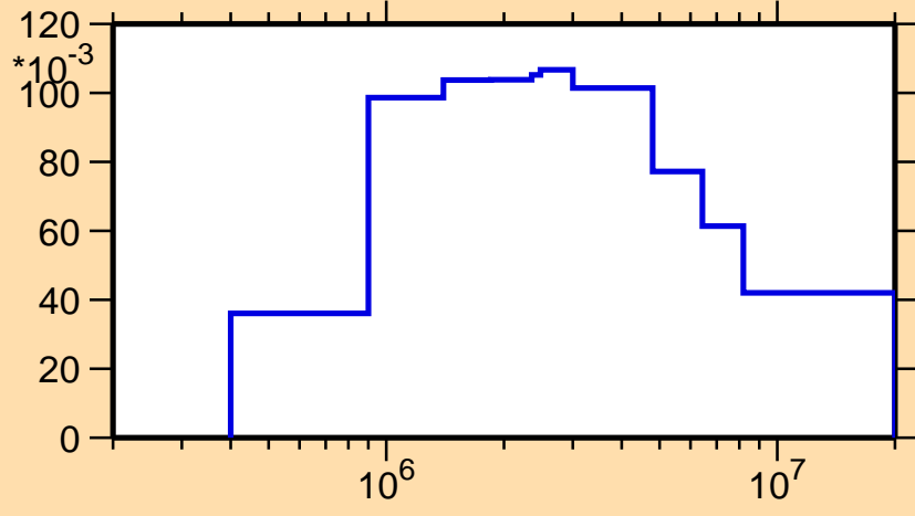
\sigma vs. E for ^{77}\text{Sr}(n,n_2)
