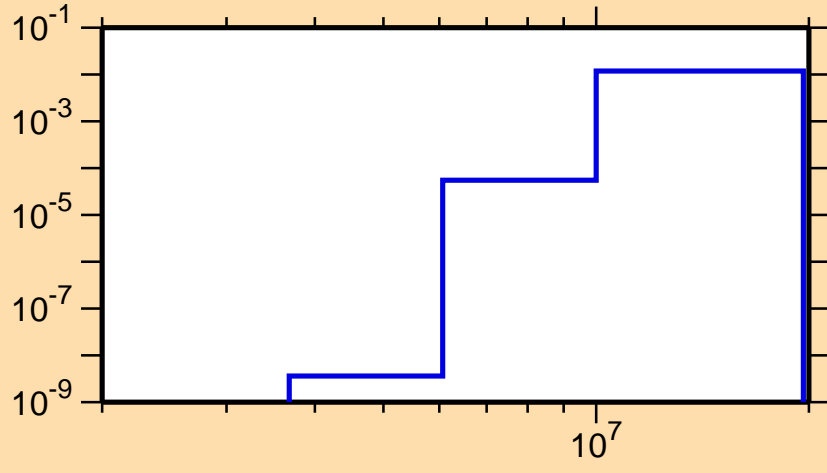
\sigma vs. E for ^{78}\text{Sr}(n,d)
