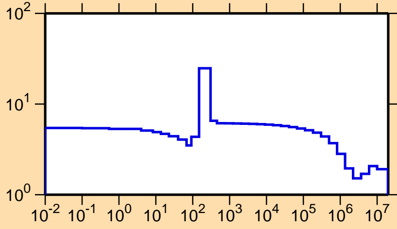
\sigma vs. E for ^{78}\text{Sr}(n,\text{el.})
