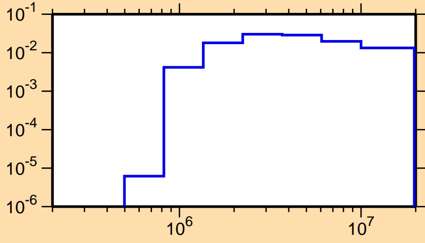
\sigma vs. E for ^{78}\text{Sr}(n,n_2)
