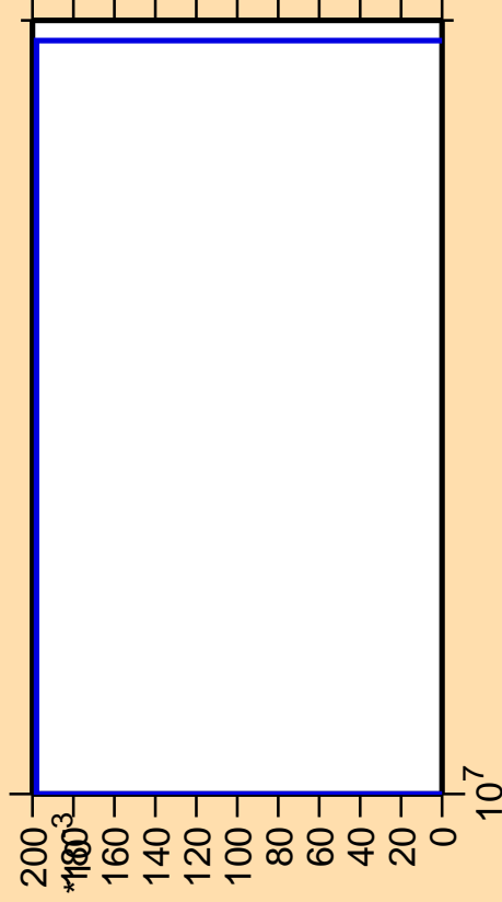
\Delta\sigma/\sigma vs. E for ^{78}\text{Sr} (mt 34)
