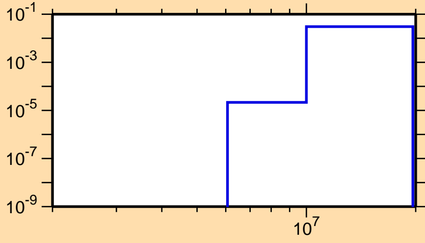
\sigma vs. E for ^{78}\text{Sr}(n,p\alpha)
