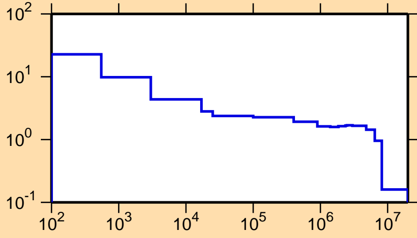
\sigma vs. E for ^{78}\text{Sr}(n,p)
