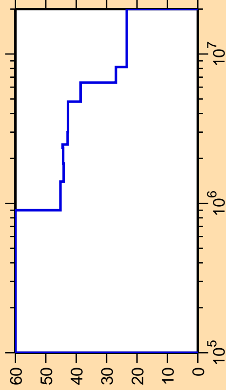
\Delta\sigma/\sigma vs. E for ^{78}\text{Sr}(n,\text{inel.})
