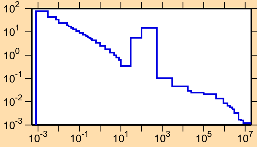
\sigma vs. E for ^{78}\text{Sr}(n,\gamma)
