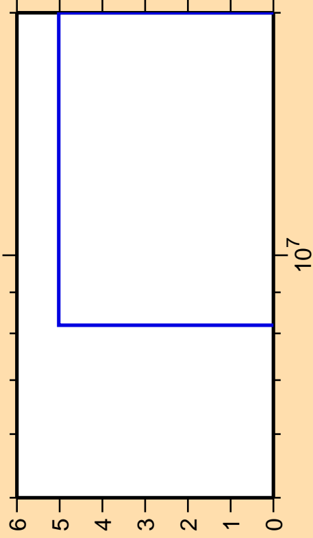
\Delta\sigma/\sigma vs. E for ^{78}\text{Sr}(n,2np)
