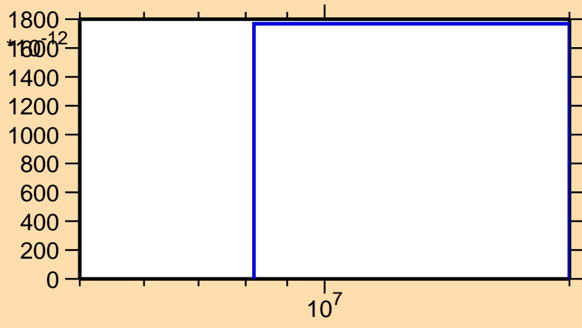
\sigma vs. E for ^{78}\text{Sr}(\text{mt } 45)
