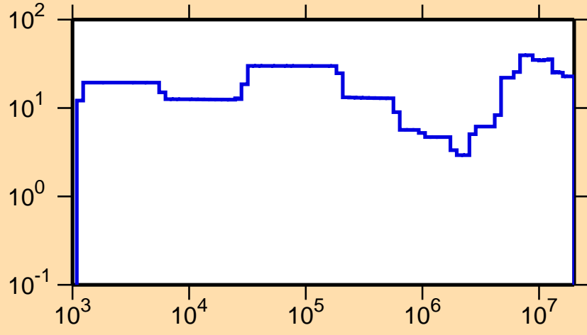
\Delta\sigma/\sigma vs. E for ^{79}\text{Sr}(n,p)
