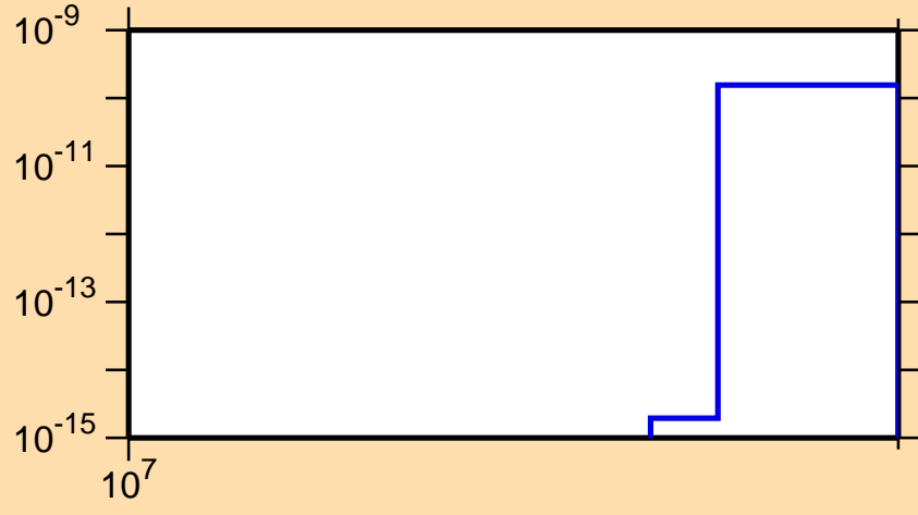
\sigma vs. E for ^{79}\text{Sr}(n,2n\alpha)
