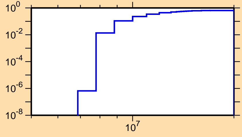
\sigma vs. E for ^{79}\text{Sr}(n,np)
