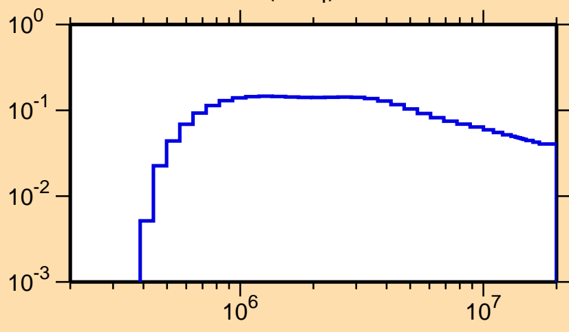
\sigma vs. E for ^{79}\text{Sr}(n,n_4)
