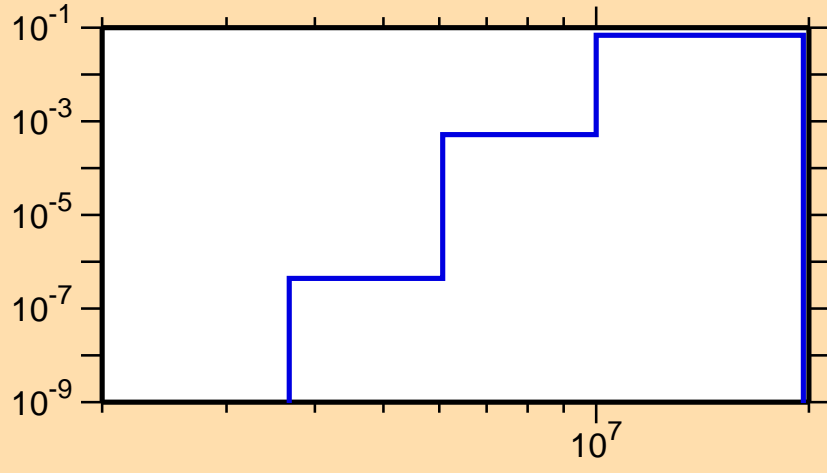
\sigma vs. E for ^{79}\text{Sr}(n,p\alpha)
