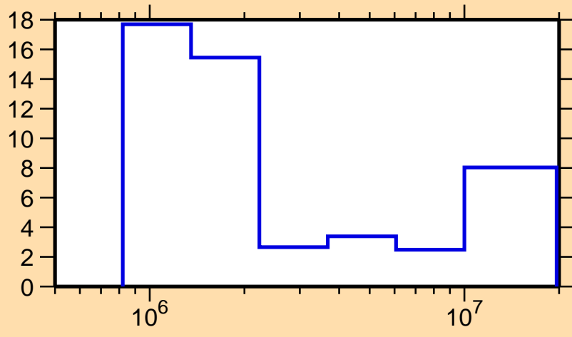
\Delta\sigma/\sigma vs. E for ^{79}\text{Sr}(n, el.)
