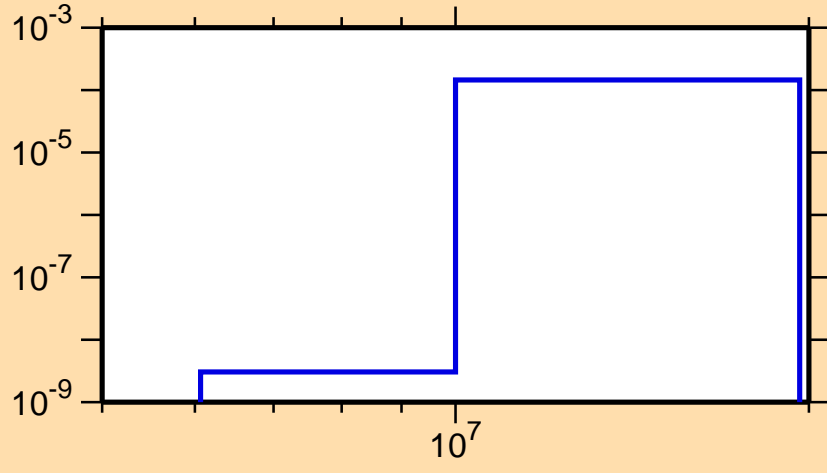
\sigma vs. E for ^{79}\text{Sr}(n,\text{He}3)
