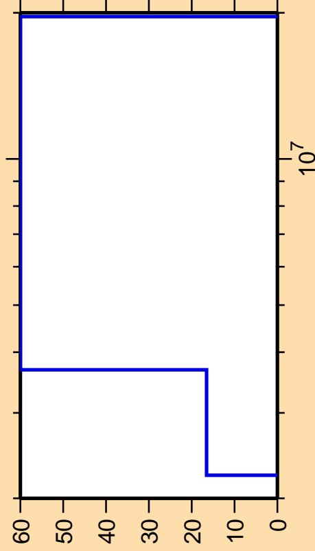
\Delta\sigma/\sigma vs. E for ^{79}\text{Sr}(n,p\alpha)
