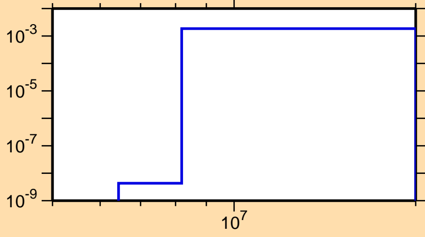
\sigma vs. E for ^{79}\text{Sr}(n,\alpha)
