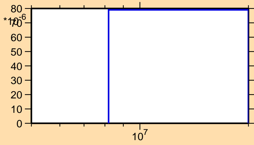
\sigma vs. E for ^{79}\text{Sr}(n,t)
