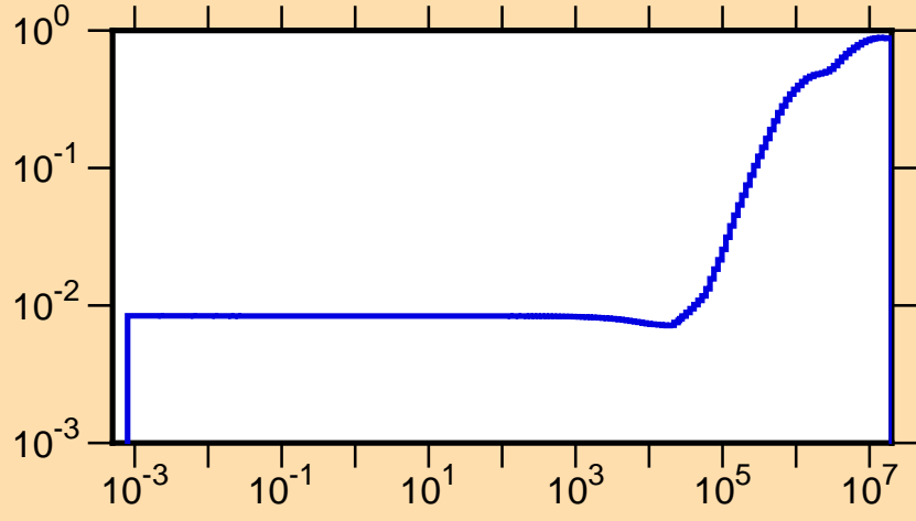
\mu vs. E for ^{80}\text{Sr}(\text{mt}251)
