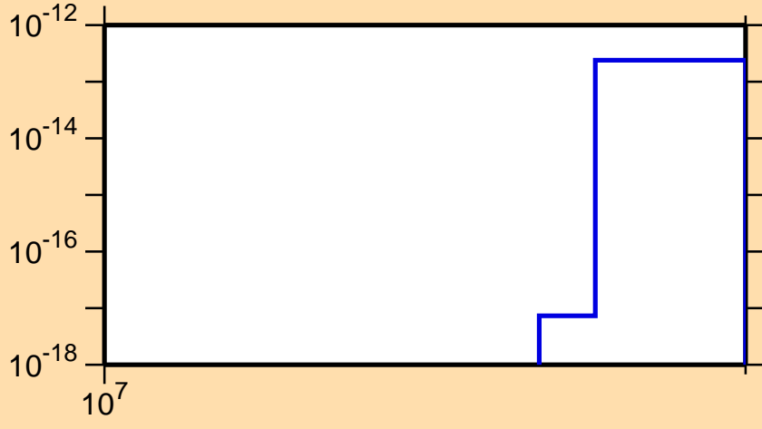
\sigma vs. E for ^{80}\text{Sr} (mt 34)
