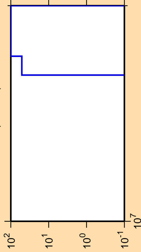
\Delta\sigma/\sigma vs. E for ^{80}\text{Sr} (mt117)
