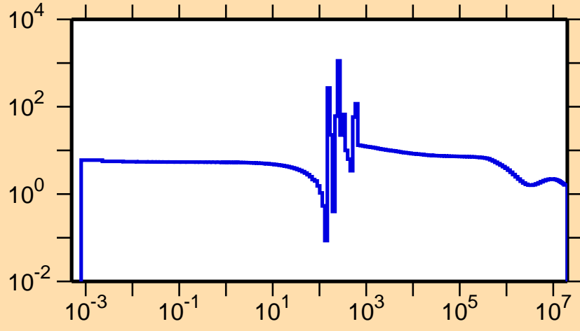
\sigma vs. E for ^{80}\text{Sr}(n,\text{el.})
