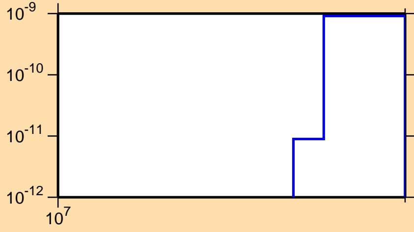
\sigma vs. E for ^{80}\text{Sr} (mt117)
