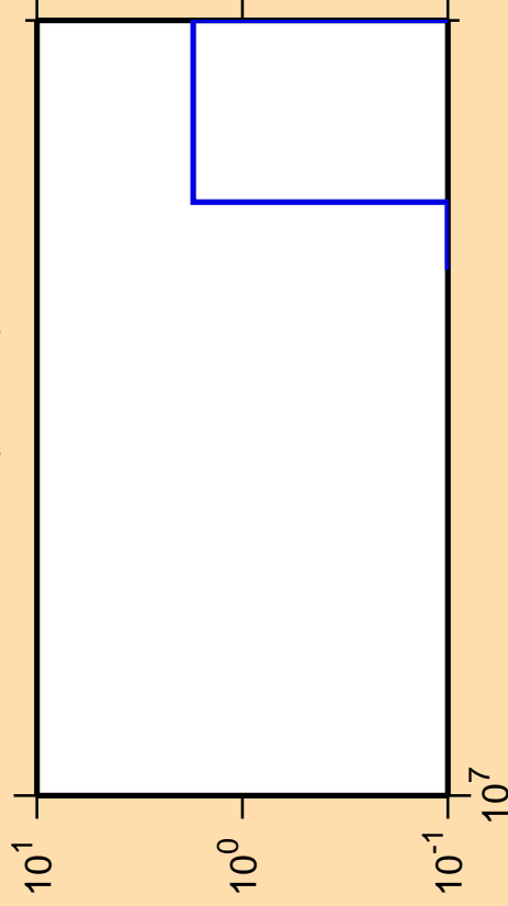
\Delta\sigma/\sigma vs. E for ^{80}\text{Sr} (mt 34)
