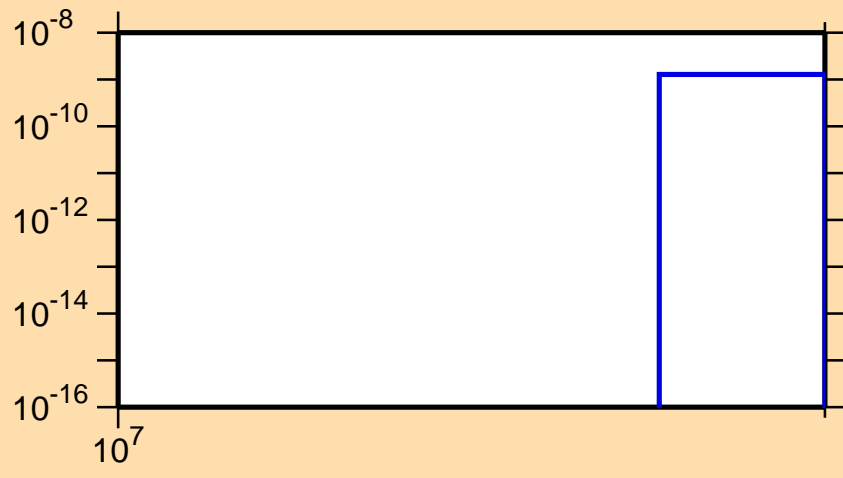
\sigma vs. E for ^{80}\text{Sr}(n,\text{pt})
