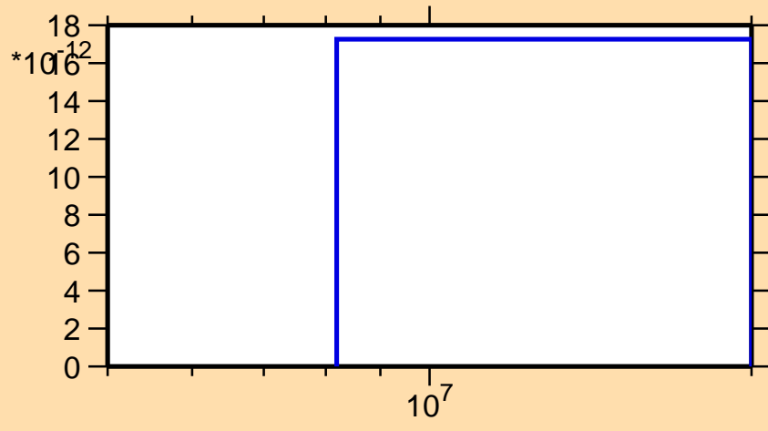
\sigma vs. E for ^{80}\text{Sr}(n,\text{nd})
