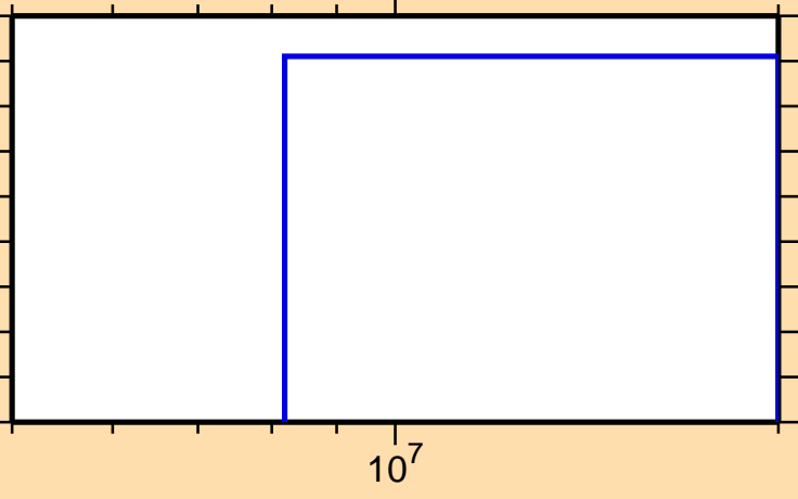
\sigma vs. E for ^{80}\text{Sr}(n,\text{pd})
