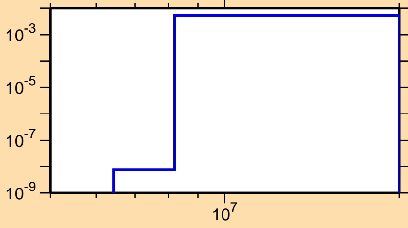
\sigma vs. E for ^{80}\text{Sr}(n,\alpha)
