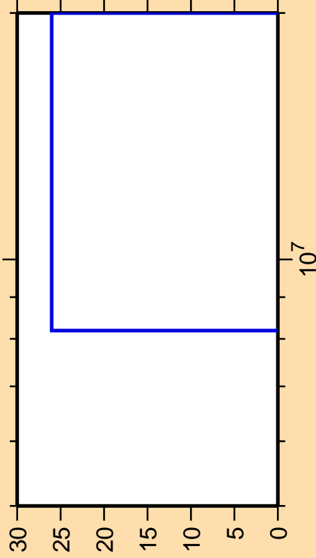
\Delta\sigma/\sigma vs. E for ^{80}\text{Sr}(n,n_1)
