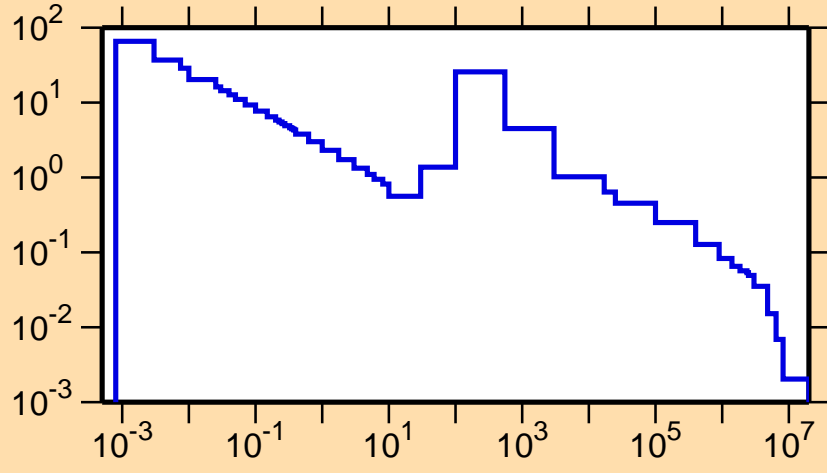
\sigma vs. E for ^{80}\text{Sr}(n,\gamma)
