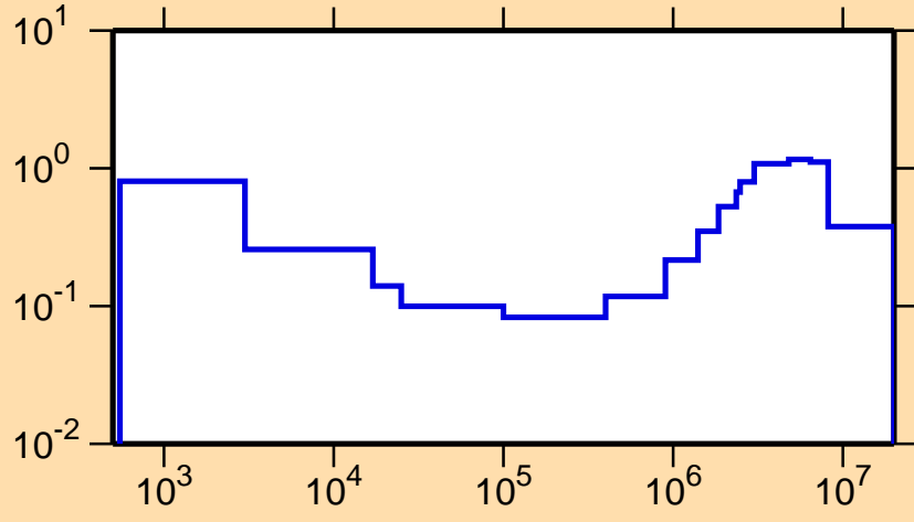
\sigma vs. E for ^{80}\text{Sr}(n,p)
