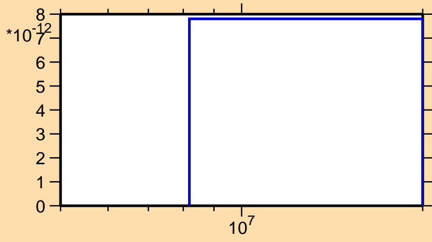
\sigma vs. E for ^{80}\text{Sr}(\text{mt117})
