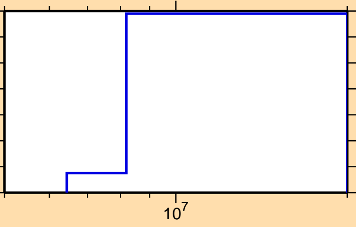
\sigma vs. E for ^{80}\text{Sr}(n,\text{He}3)
