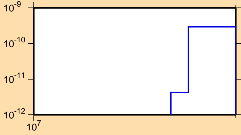
\sigma vs. E for ^{81}\text{Sr} (mt117)
