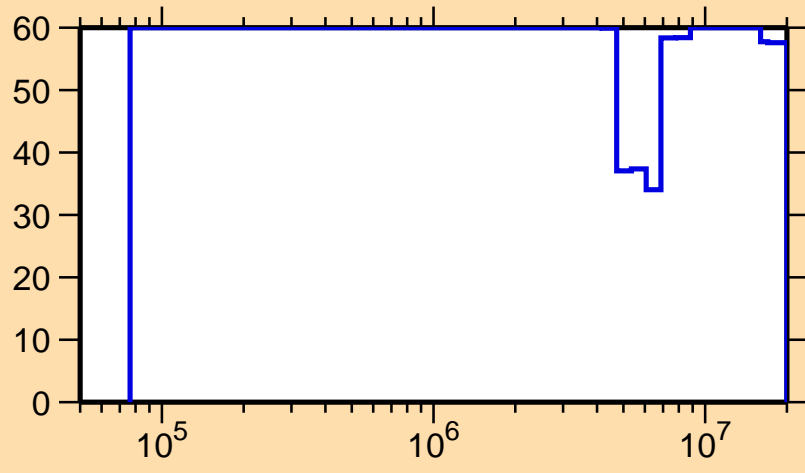
\Delta\sigma/\sigma vs. E for ^{81}\text{Sr}(n,n_1)
