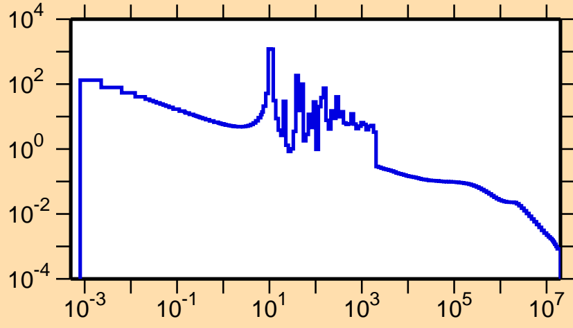
\sigma vs. E for ^{81}\text{Sr}(n,\gamma)
