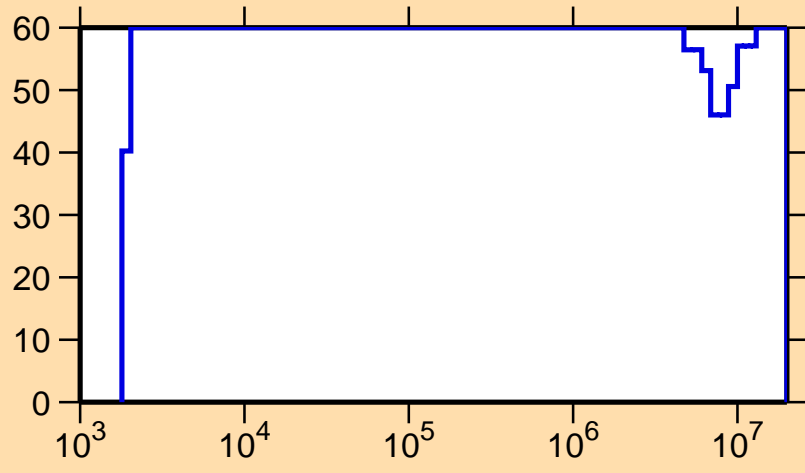
\Delta\sigma/\sigma vs. E for ^{81}\text{Sr}(n,\gamma)
