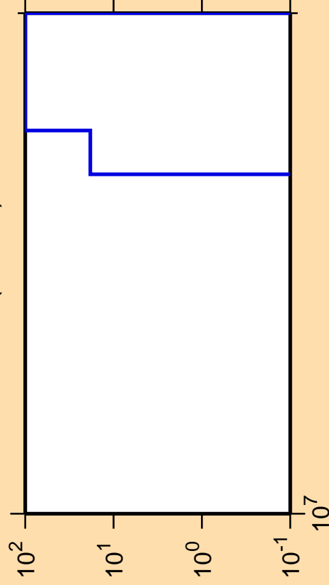
\Delta\sigma/\sigma vs. E for ^{81}\text{Sr} (mt117)
