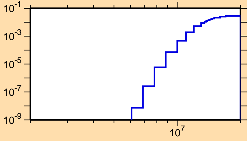
\sigma vs. E for ^{81}\text{Sr}(n,p\alpha)
