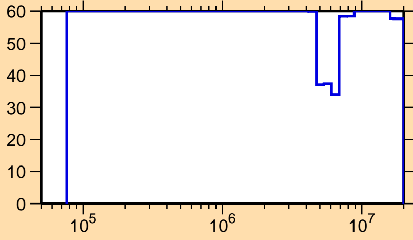
\Delta\sigma/\sigma vs. E for ^{81}\text{Sr}(n,n_1)
