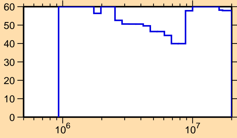
\Delta\sigma/\sigma vs. E for ^{81}\text{Sr}(n,n\text{cont.})
