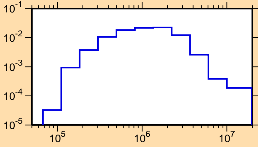
\sigma vs. E for ^{81}\text{Sr}(n,n_2)
