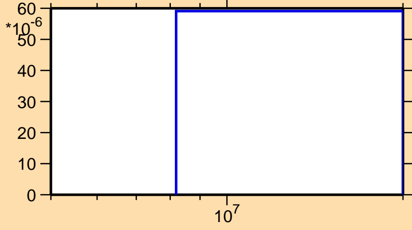
\sigma vs. E for ^{81}\text{Sr}(n,t)
