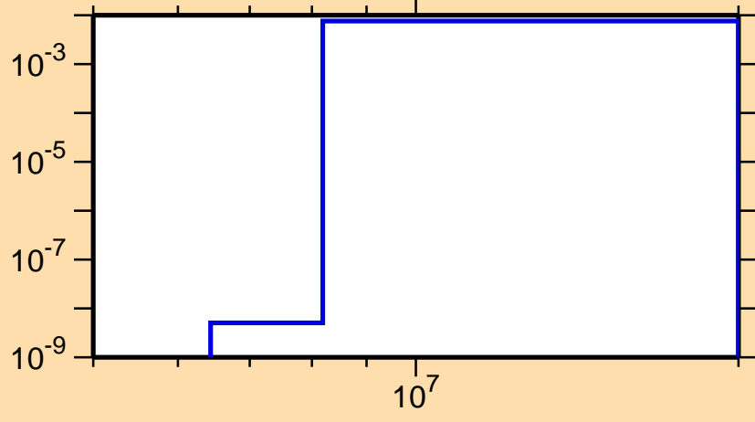
\sigma vs. E for ^{81}\text{Sr}(n,\alpha)
