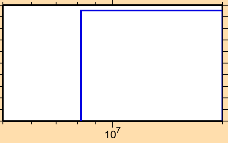
\sigma vs. E for ^{81}\text{Sr}(n,\text{pt})
