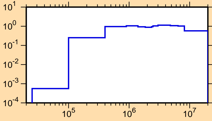
\sigma vs. E for ^{81}\text{Sr}(n,\text{inel.})
