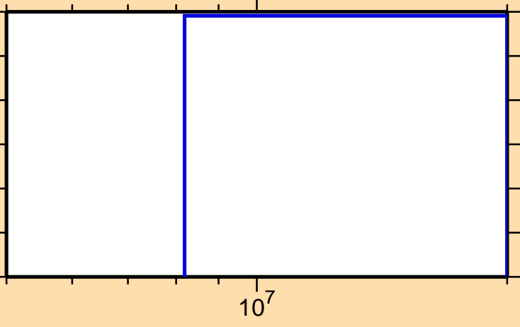
\sigma vs. E for ^{81}\text{Sr}(n,t)
