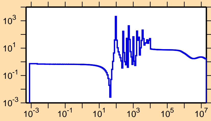
\sigma vs. E for ^{82}\text{Sr}(n,\text{el.})
