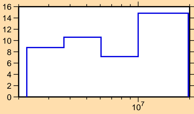
\Delta\sigma/\sigma vs. E for ^{82}\text{Sr}(n,el.)
