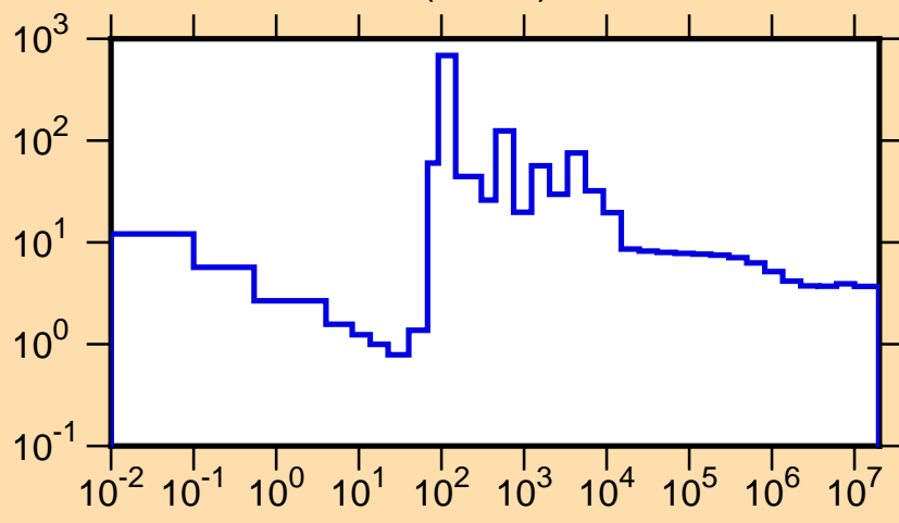
\sigma vs. E for ^{82}\text{Sr}(n,\text{tot.})
