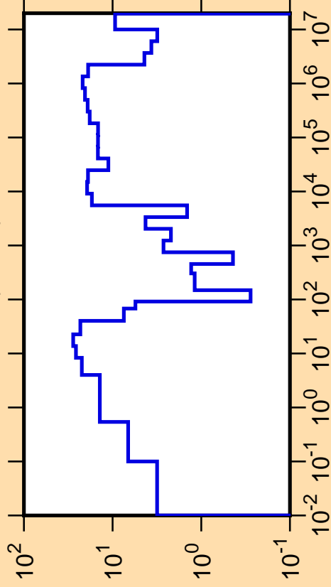
\Delta\sigma/\sigma vs. E for ^{82}\text{Sr}(n,\text{tot.})
