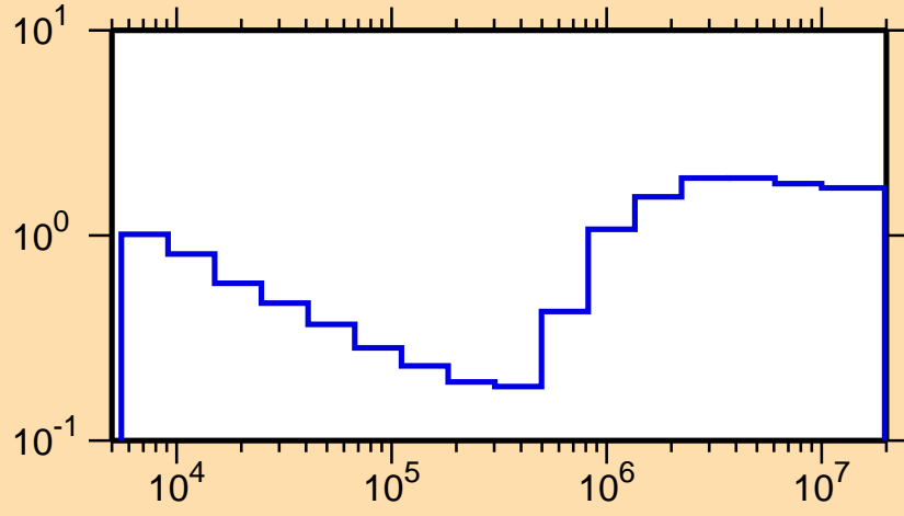
\sigma vs. E for ^{82}\text{Sr}(n,\text{nonel.})
