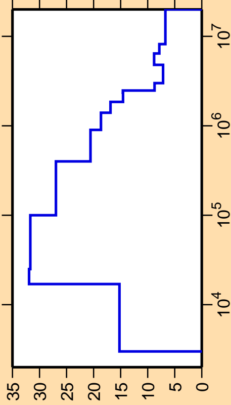
\Delta\sigma/\sigma vs. E for ^{82}\text{Sr}(n,\text{nonel.})
