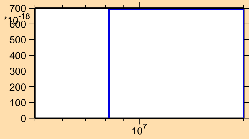
\sigma vs. E for ^{82}\text{Sr}(n,\text{pt})
