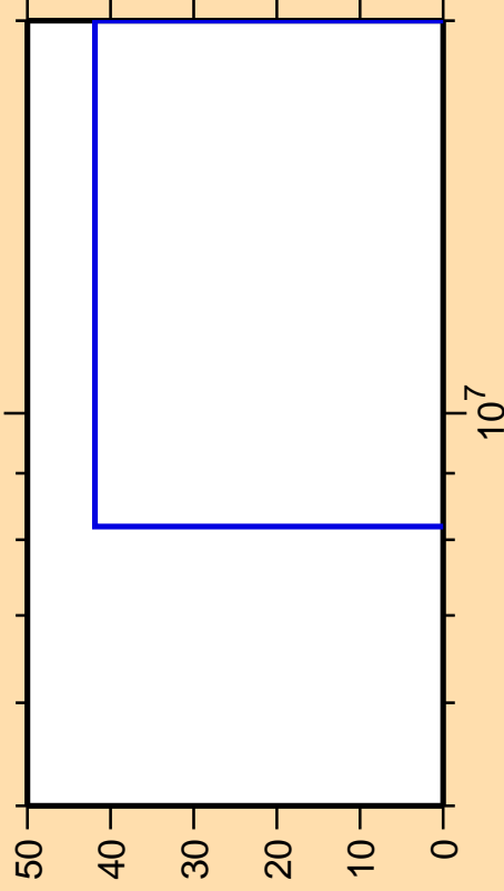
\Delta\sigma/\sigma vs. E for ^{82}\text{Sr}(n,\gamma)
