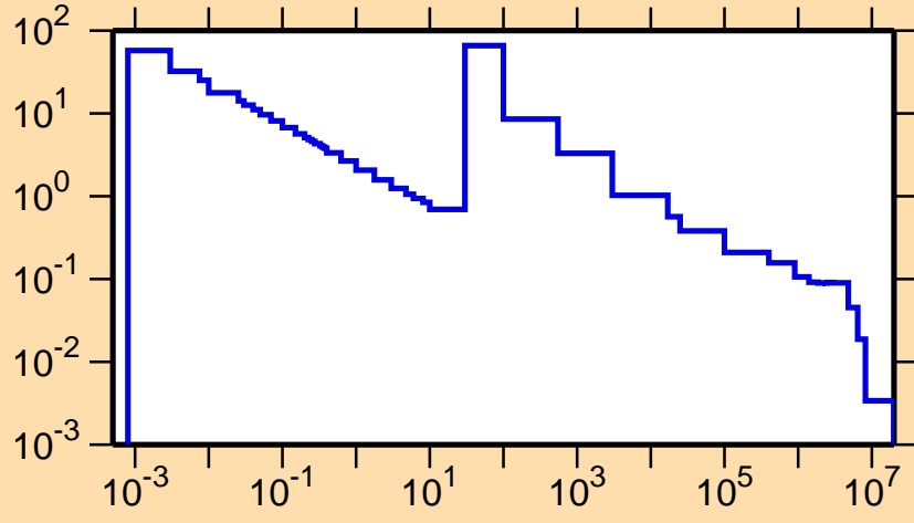
\sigma vs. E for ^{82}\text{Sr}(n,\gamma)
