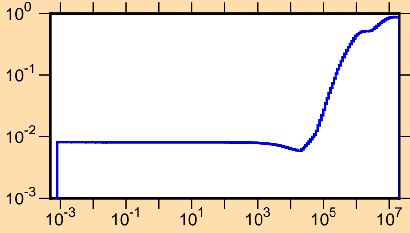
\mu vs. E for ^{83}\text{Sr}(\text{mt251})
