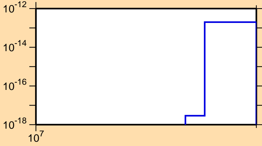
\sigma vs. E for ^{83}\text{Sr} (mt117)
