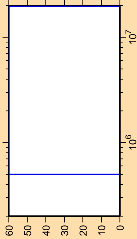
\Delta\sigma/\sigma vs. E for ^{83}\text{Sr}(n,n_4)
