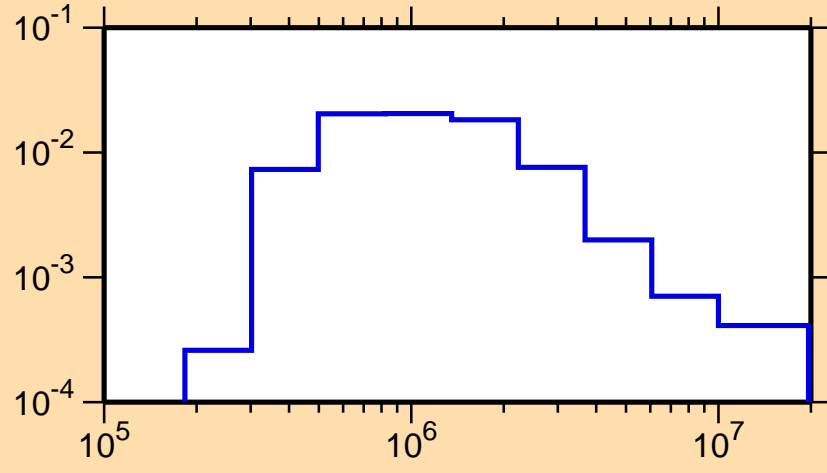
\sigma vs. E for ^{83}\text{Sr}(n,n_2)
