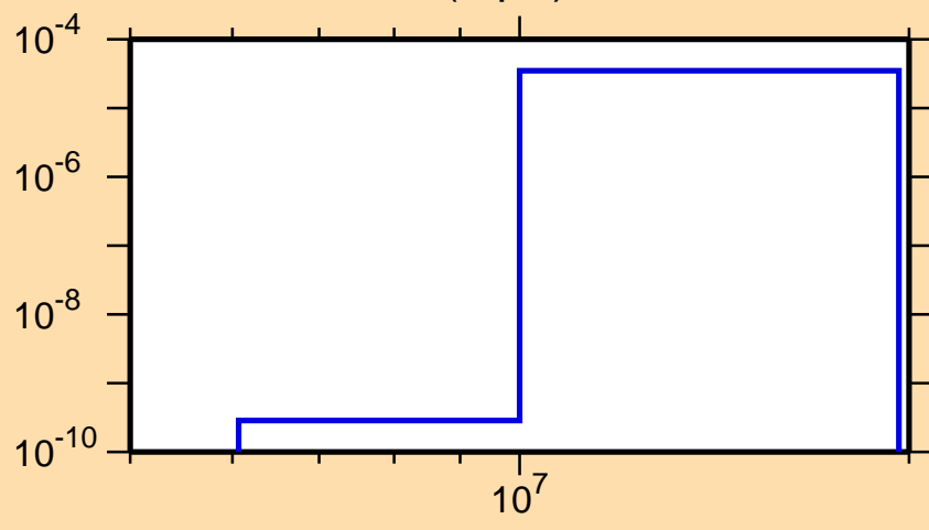
\sigma vs. E for ^{83}\text{Sr}(n,p\alpha)
