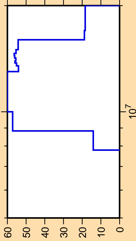
\Delta\sigma/\sigma vs. E for ^{83}\text{Sr}(n,n_{\text{cont}}) .
