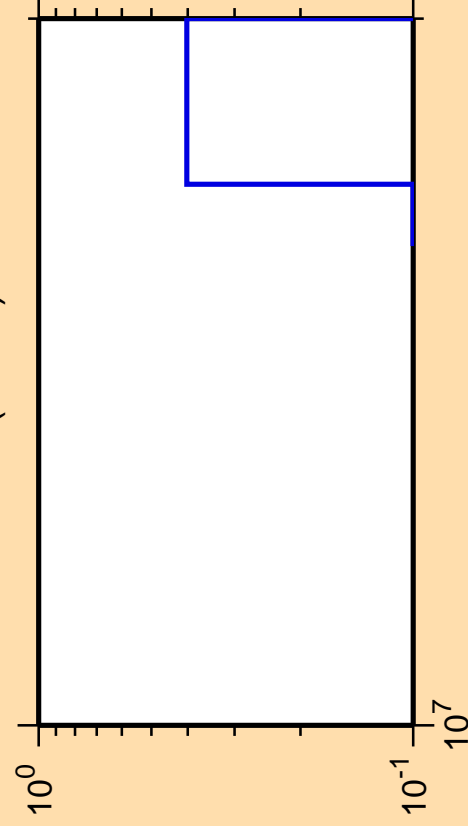
\Delta\sigma/\sigma vs. E for ^{83}\text{Sr} (mt 45)
