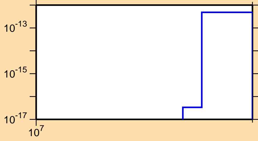
\sigma vs. E for ^{83}\text{Sr} (mt117)
