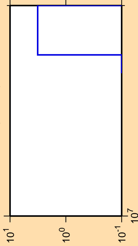
\Delta\sigma/\sigma vs. E for ^{83}\text{Sr} (mt117)
