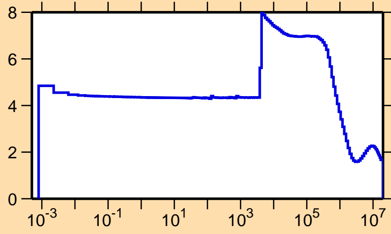
\sigma vs. E for ^{83}\text{Sr}(n,\text{el.})
