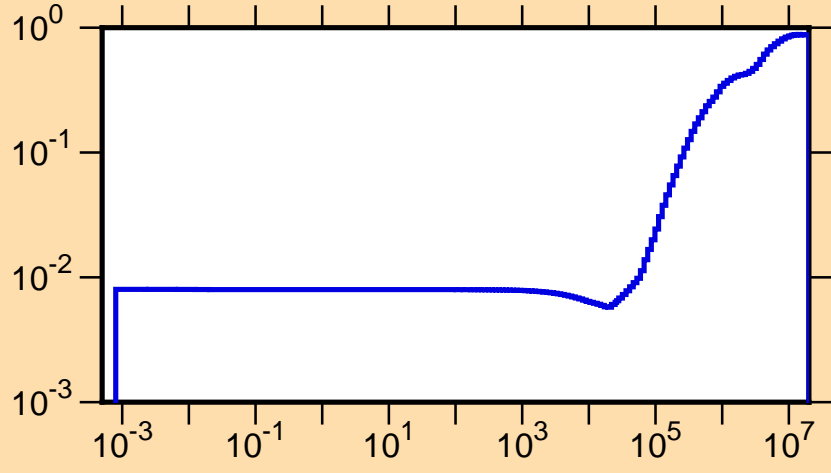
\mu vs. E for ^{84}\text{Sr}(\text{mt251})
