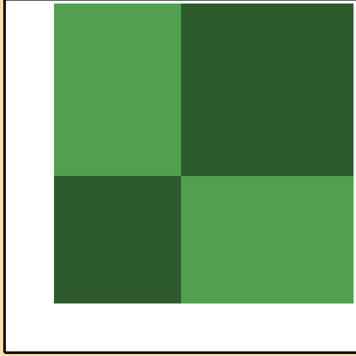
\sigma vs. E for ^{84}\text{Sr}(n,\alpha)
