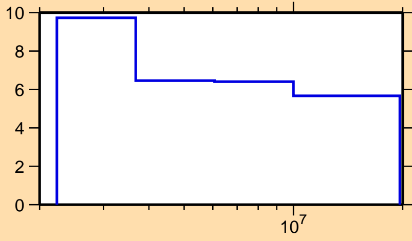
\Delta\sigma/\sigma vs. E for ^{84}\text{Sr}(n,n\text{onel.})
