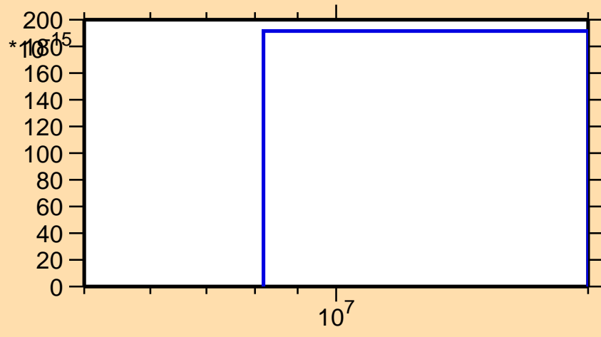
\sigma vs. E for ^{84}\text{Sr}(n,\text{nd})
