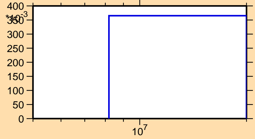
\sigma vs. E for ^{84}\text{Sr}(n,2n)
