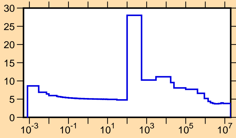
\sigma vs. E for ^{84}\text{Sr}(n,\text{tot.})
