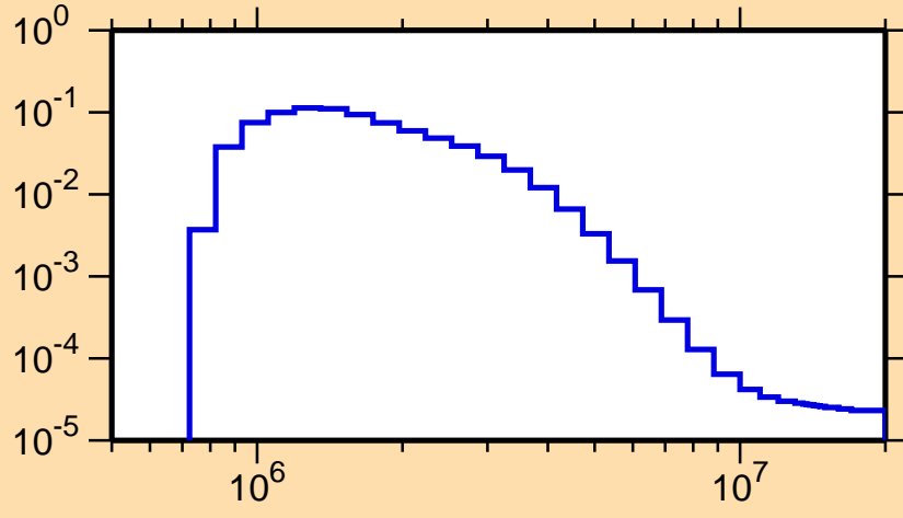
\sigma vs. E for ^{85}\text{Sr}(n,n_4)
