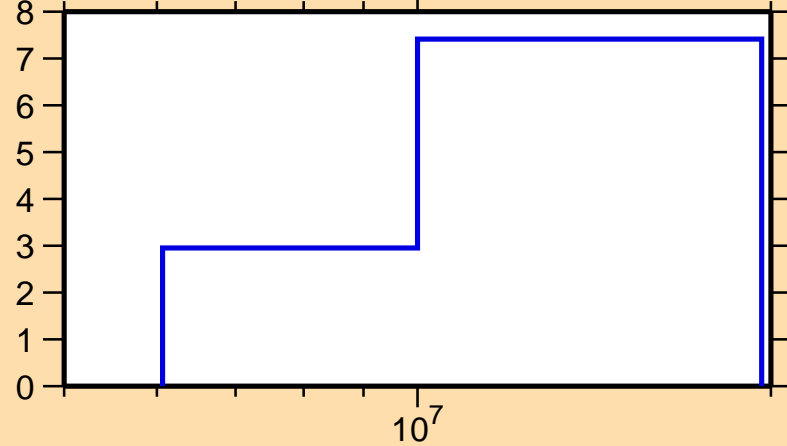
\Delta\sigma/\sigma vs. E for ^{85}\text{Sr}(n,\text{tot.})
