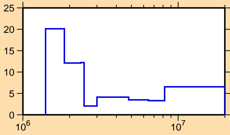
\Delta\sigma/\sigma vs. E for ^{85}\text{Sr}(n,tot.)
