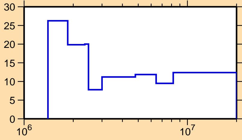
\Delta\sigma/\sigma vs. E for ^{85}\text{Sr}(n, el.)
