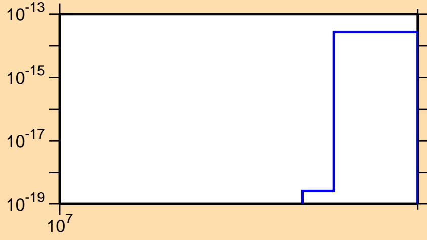
\sigma vs. E for ^{85}\text{Sr} (mt 34)
