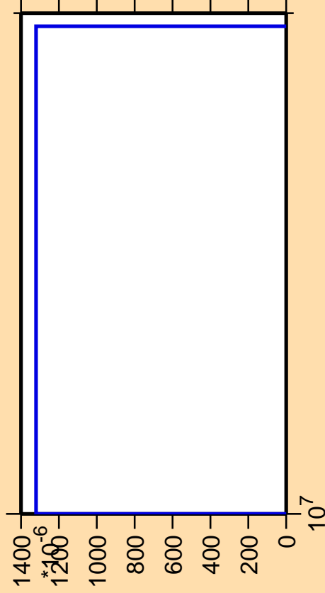
\Delta\sigma/\sigma vs. E for ^{85}\text{Sr} (mt 34)
