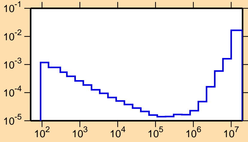
\sigma vs. E for ^{85}\text{Sr}(n,\alpha)
