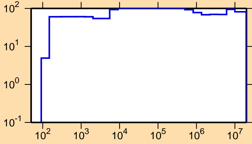
\Delta\sigma/\sigma vs. E for ^{85}\text{Sr}(n,p)
