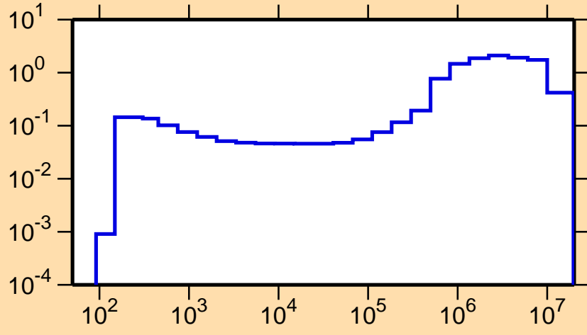
\sigma vs. E for ^{85}\text{Sr}(n,\text{inel.})
