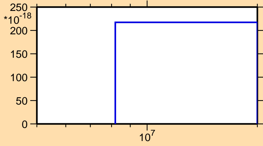
\sigma vs. E for ^{85}\text{Sr} (mt 34)
