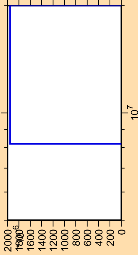
\Delta\sigma/\sigma vs. E for ^{85}\text{Sr} (mt 34)
