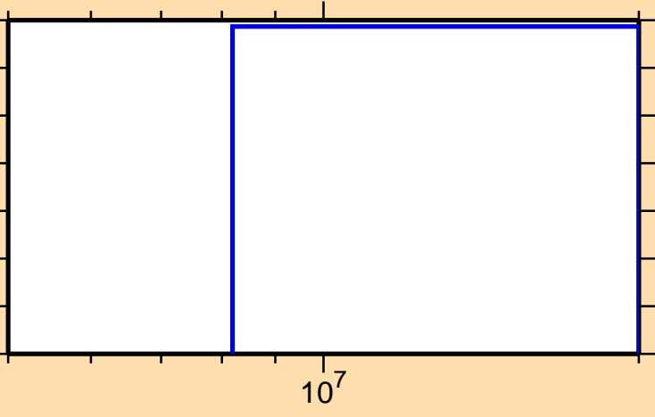
\sigma vs. E for ^{85}\text{Sr}(n,\text{He3})
