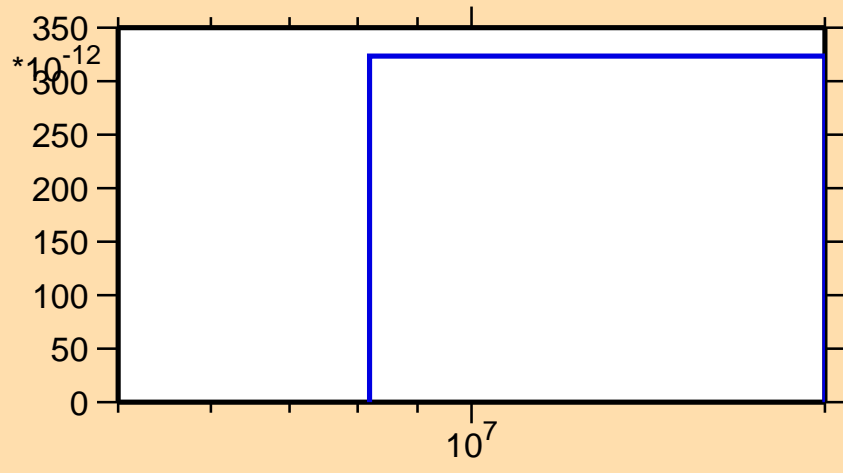
\sigma vs. E for ^{85}\text{Sr}(n,2n\alpha)
