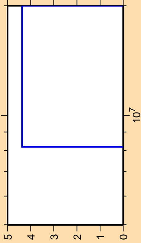
\Delta\sigma/\sigma vs. E for ^{85}\text{Sr}(n,\text{pt})
