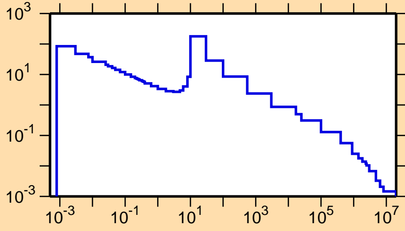
\sigma vs. E for ^{85}\text{Sr}(n,\gamma)
