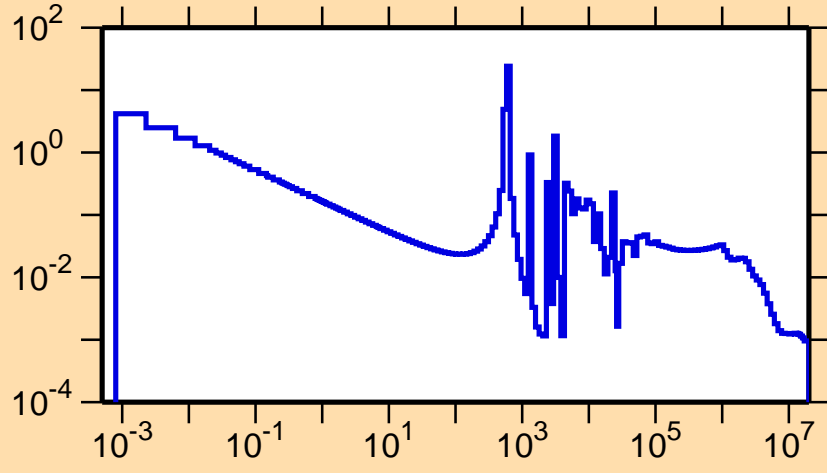
\sigma vs. E for ^{86}\text{Sr}(n,\gamma)
