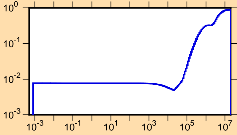
\mu vs. E for ^{87}\text{Sr}(\text{mt251})
