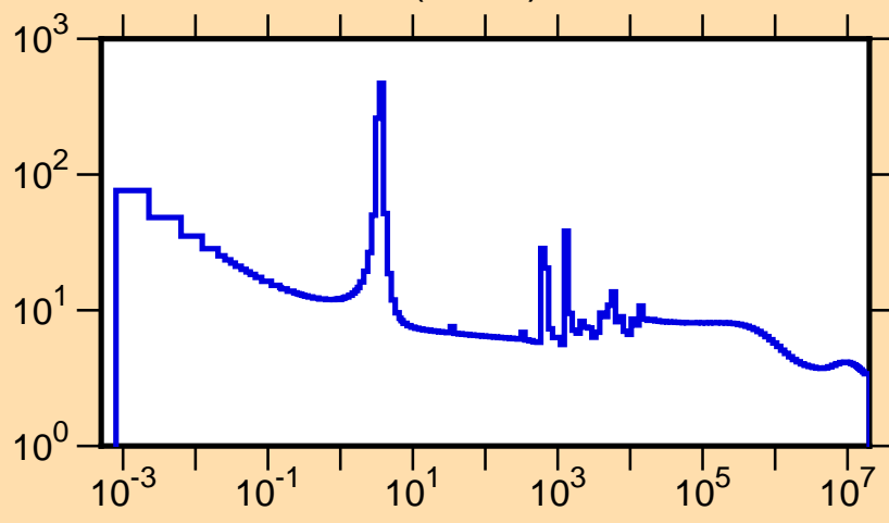
\sigma vs. E for ^{87}\text{Sr}(n,\text{tot.})
