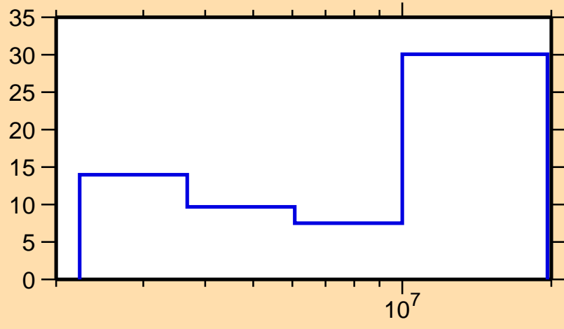
\Delta\sigma/\sigma vs. E for ^{87}\text{Sr}(n,ncont.)
