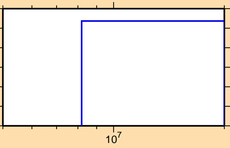
\sigma vs. E for ^{87}\text{Sr}(n,2np)
