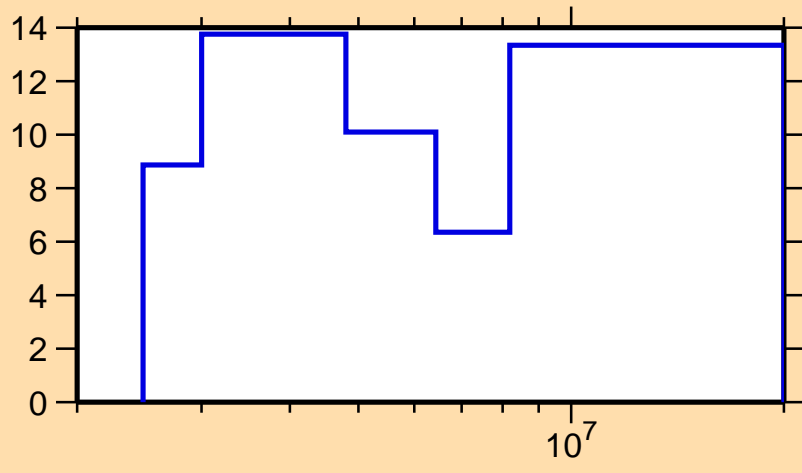
\Delta\sigma/\sigma vs. E for ^{87}\text{Sr}(n, el.)
