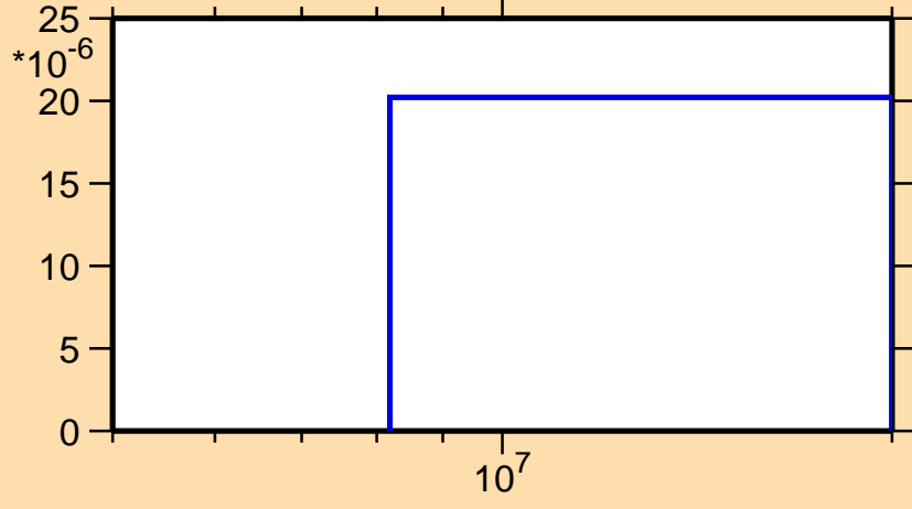
\sigma vs. E for ^{87}\text{Sr}(n,t)
