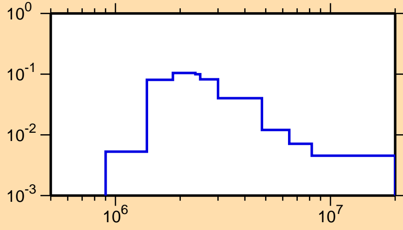
\sigma vs. E for ^{87}\text{Sr}(n,n_4)
