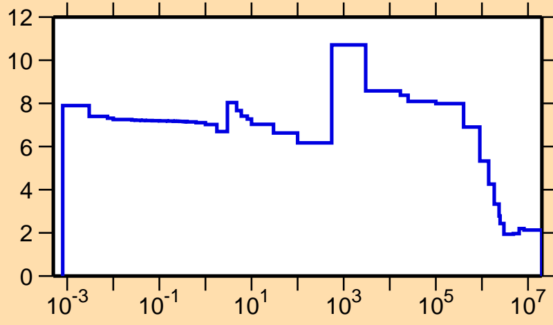
\sigma vs. E for ^{87}\text{Sr}(n,\text{el.})
