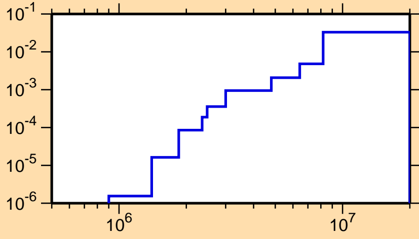
\sigma vs. E for ^{87}\text{Sr}(n,p)
