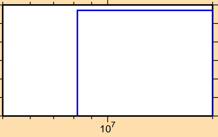
\sigma vs. E for ^{87}\text{Sr}(n,np)
