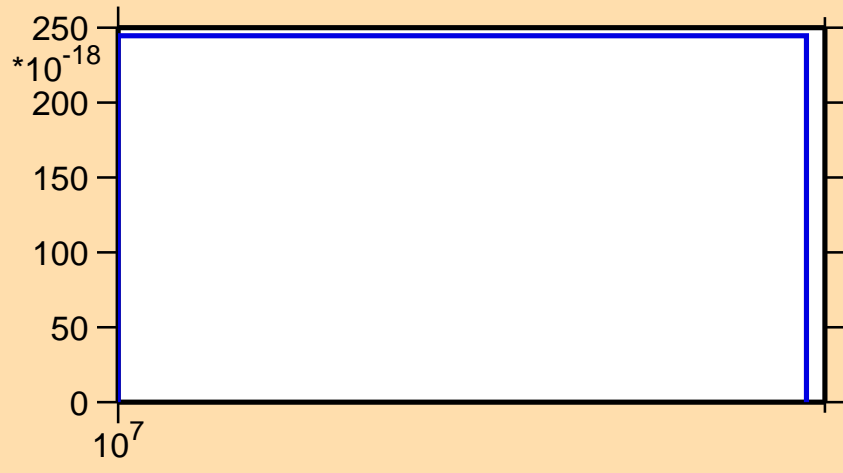
\sigma vs. E for ^{88}\text{Sr}(n,p\alpha)
