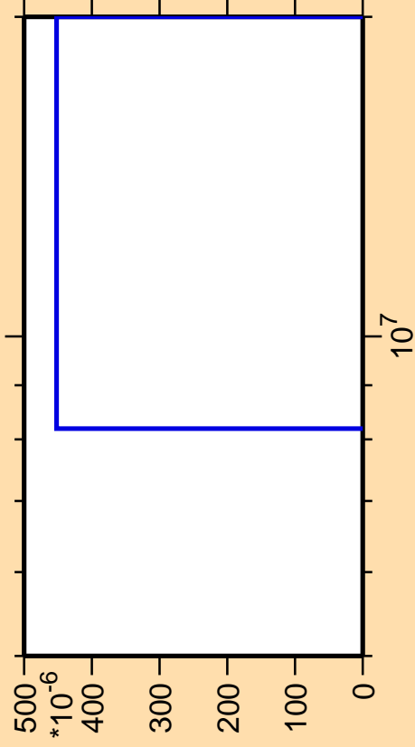
\Delta\sigma/\sigma vs. E for ^{88}\text{Sr}(n,p\alpha)
