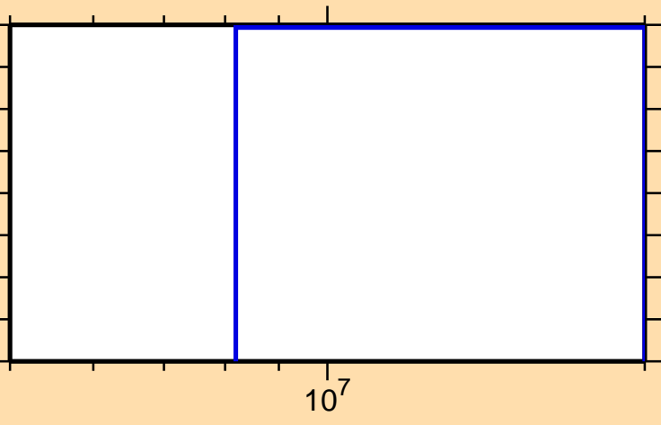
\sigma vs. E for ^{89}\text{Sr}(n,p\alpha)
