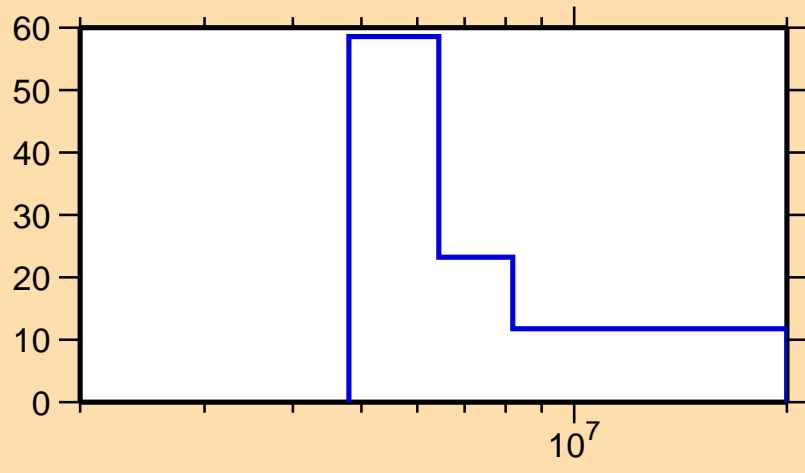
\Delta\sigma/\sigma vs. E for ^{89}\text{Sr}(n,2n)
