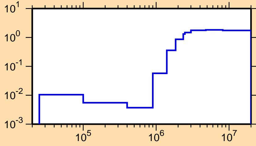
\sigma vs. E for ^{89}\text{Sr}(n,\text{nonel.})
