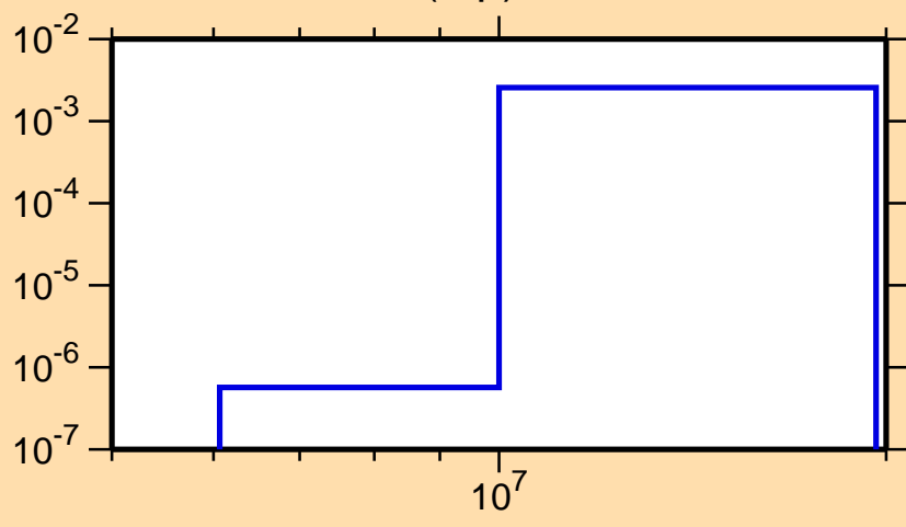
\sigma vs. E for ^{90}\text{Sr}(n,p)
