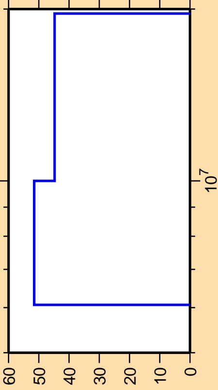
\Delta\sigma/\sigma vs. E for ^{90}\text{Sr}(n,n_1)
