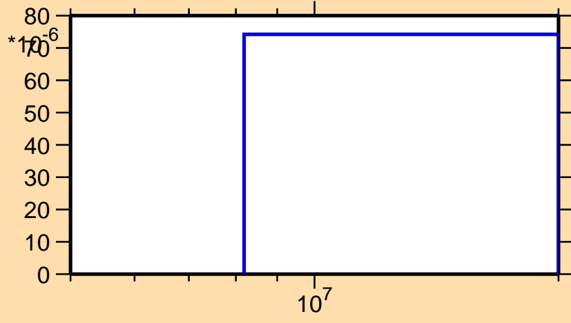
\sigma vs. E for ^{90}\text{Sr}(n,d)
