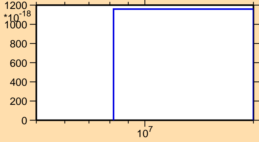
\sigma vs. E for ^{90}\text{Sr}(n,2np)
