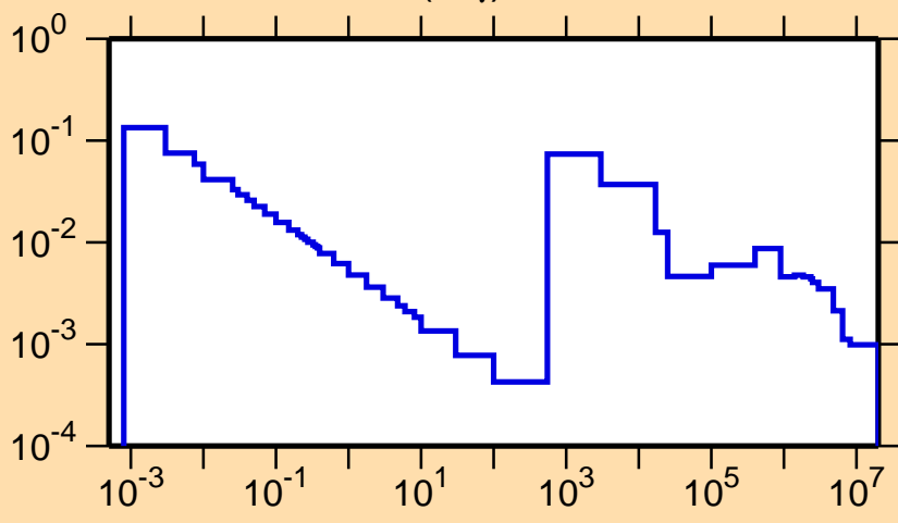
\sigma vs. E for ^{90}\text{Sr}(n,\gamma)
