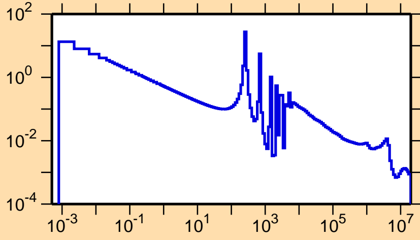
\sigma vs. E for ^{91}\text{Sr}(n,\gamma)
