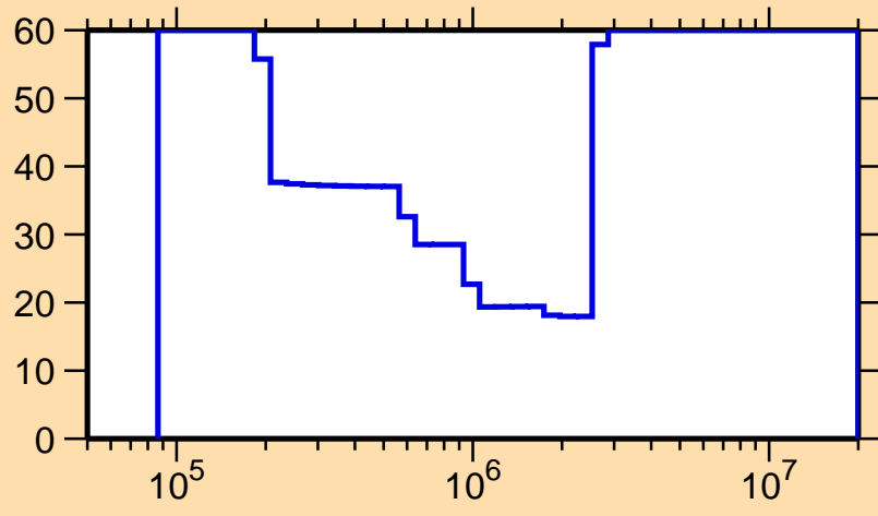
\Delta\sigma/\sigma vs. E for ^{91}\text{Sr}(n,n_1)
