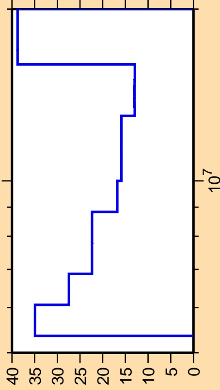
\Delta\sigma/\sigma vs. E for ^{91}\text{Sr}(n,2n)
