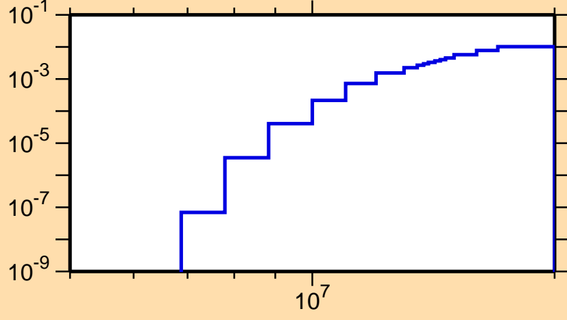
\sigma vs. E for ^{91}\text{Sr}(n,p)
