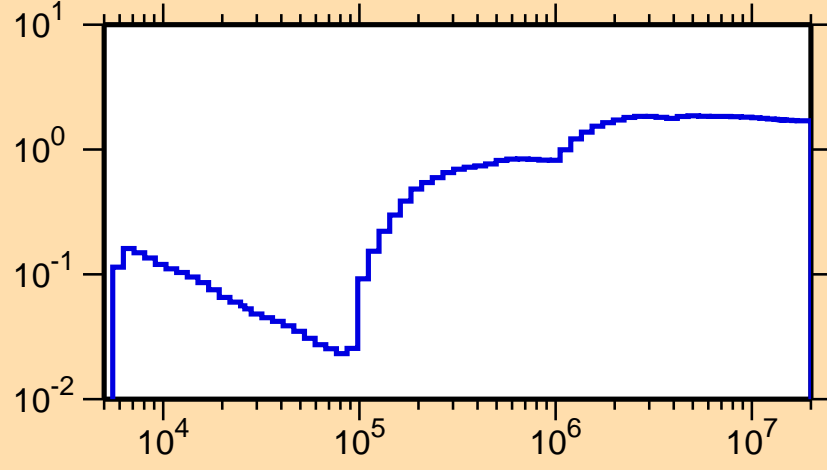
\sigma vs. E for ^{91}\text{Sr}(n,\text{nonel.})
