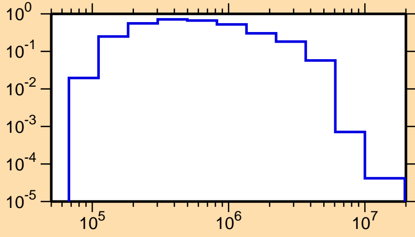
\sigma vs. E for ^{91}\text{Sr}(n,n_1)
