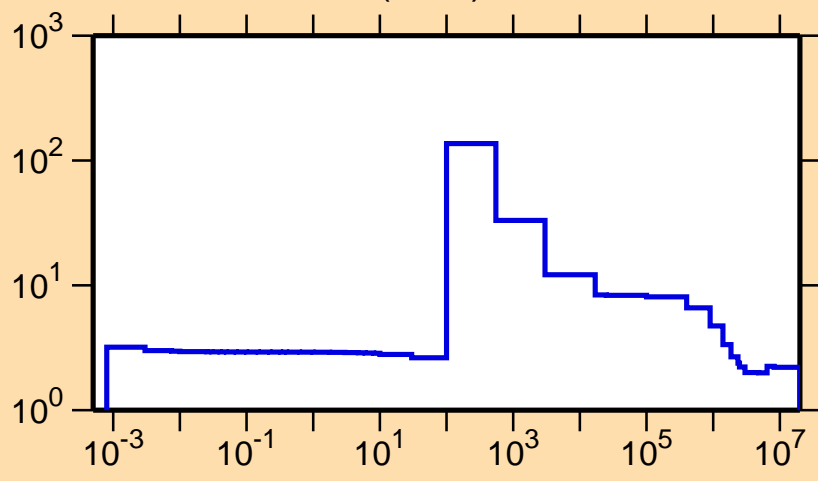
\sigma vs. E for ^{91}\text{Sr}(n,\text{el.})
