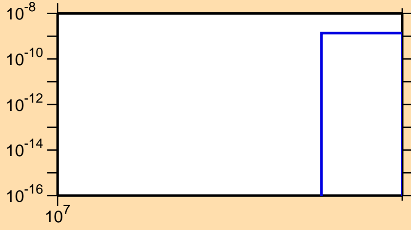
\sigma vs. E for ^{92}\text{Sr}(n,\text{nd})
