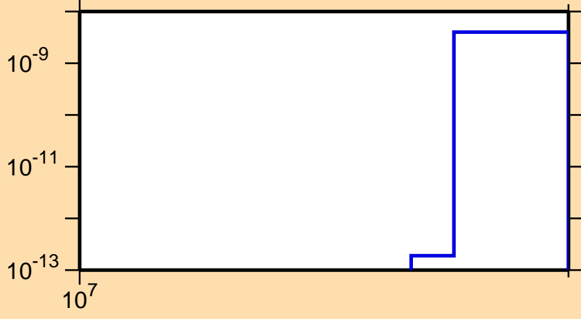
\sigma vs. E for ^{92}\text{Sr}(n,nt)
