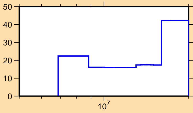
\Delta\sigma/\sigma vs. E for ^{92}\text{Sr}(n,2n)
