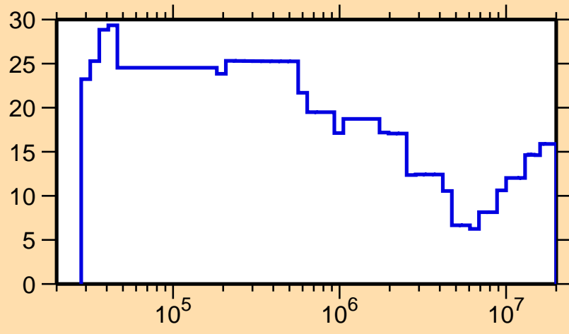
\Delta\sigma/\sigma vs. E for ^{92}\text{Sr}(n,\text{tot.})
