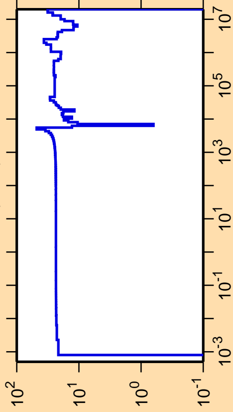
\Delta\sigma/\sigma vs. E for ^{92}\text{Sr}(n,\text{el.})
