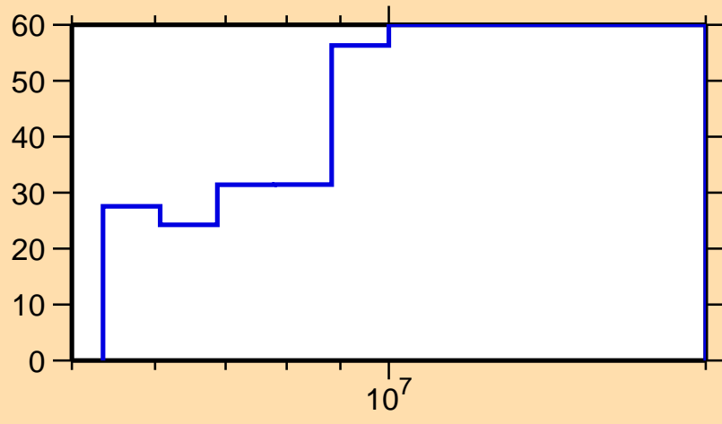
\Delta\sigma/\sigma vs. E for ^{92}\text{Sr}(n,n\text{cont.})
