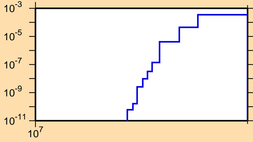
\sigma vs. E for ^{92}\text{Sr}(n,np)
