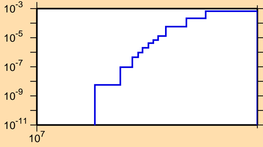
\sigma vs. E for ^{92}\text{Sr}(n,d)
