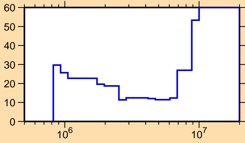
\Delta\sigma/\sigma vs. E for ^{92}\text{Sr}(n,\text{inel.})
