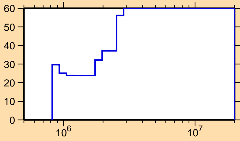
\Delta\sigma/\sigma vs. E for ^{92}\text{Sr}(n,n_1)
