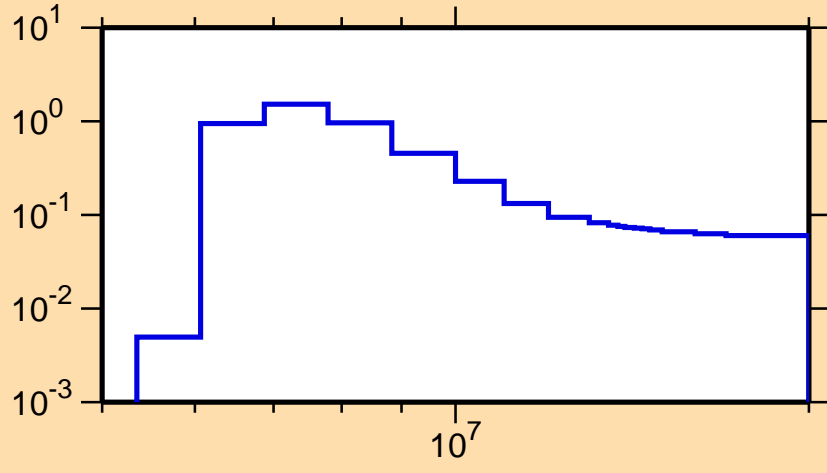
\sigma vs. E for ^{92}\text{Sr}(n,n\text{cont.})
