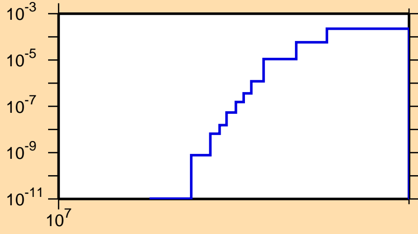
\sigma vs. E for ^{92}\text{Sr}(n,t)
