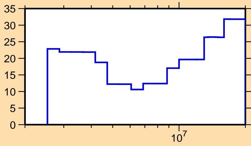
\Delta\sigma/\sigma vs. E for ^{92}\text{Sr}(n,\text{el.})
