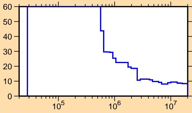
\Delta\sigma/\sigma vs. E for ^{92}\text{Sr}(n,\text{nonel.})
