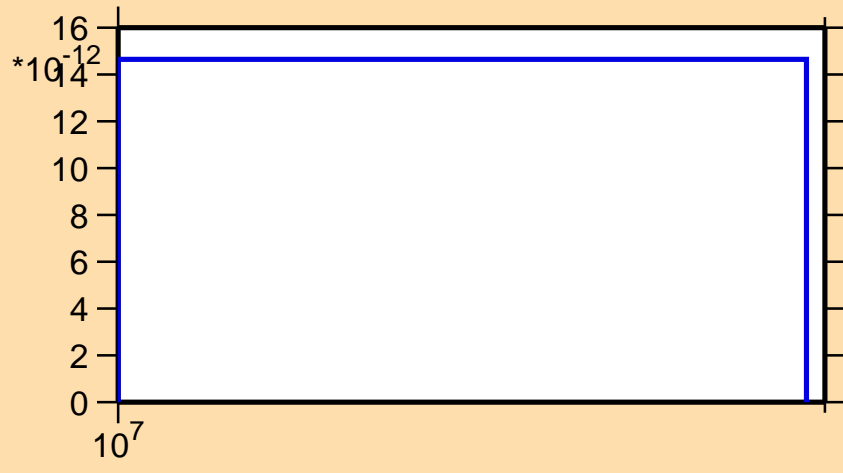
\sigma vs. E for ^{92}\text{Sr}(n,2n\alpha)
