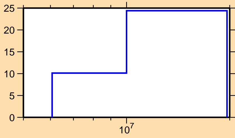
\Delta\sigma/\sigma vs. E for ^{92}\text{Sr}(n,el.)
