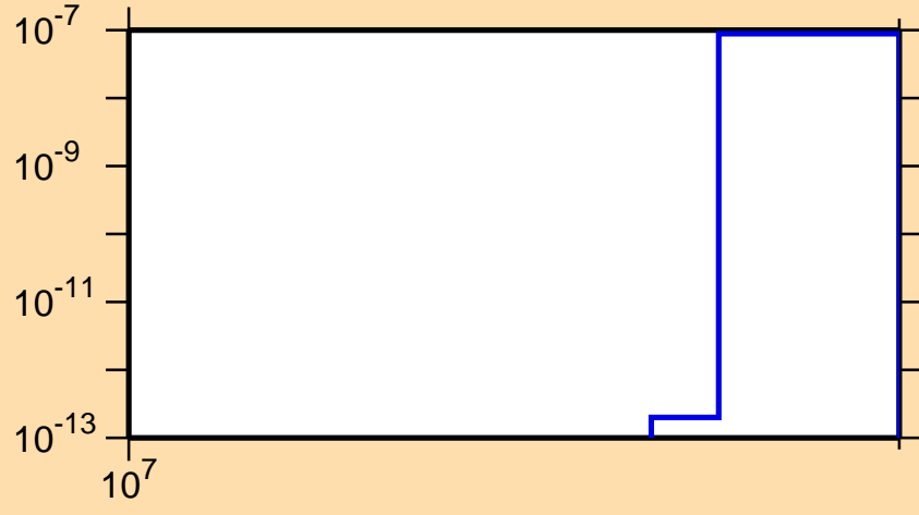
\sigma vs. E for ^{93}\text{Sr}(n,\text{nd})
