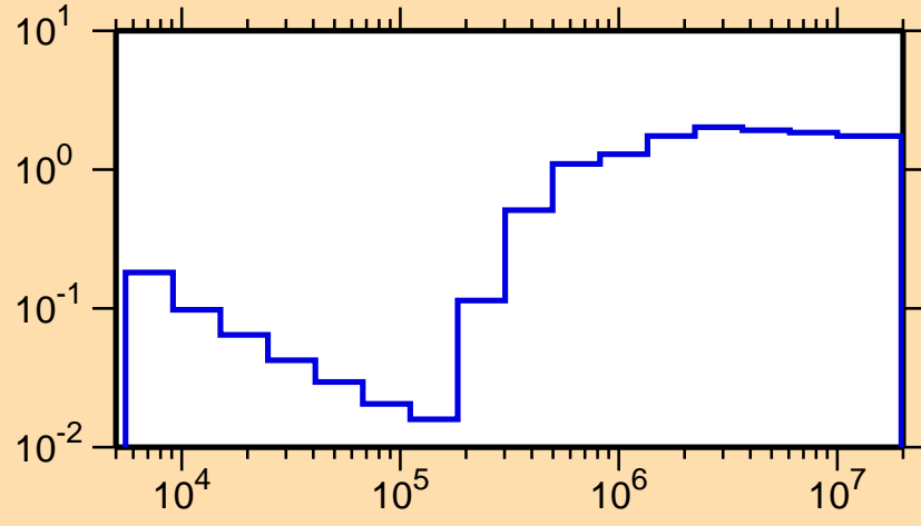
\sigma vs. E for ^{93}\text{Sr}(n,\text{nonel.})
