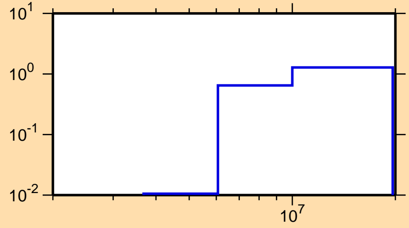
\sigma vs. E for ^{93}\text{Sr}(n,2n)
